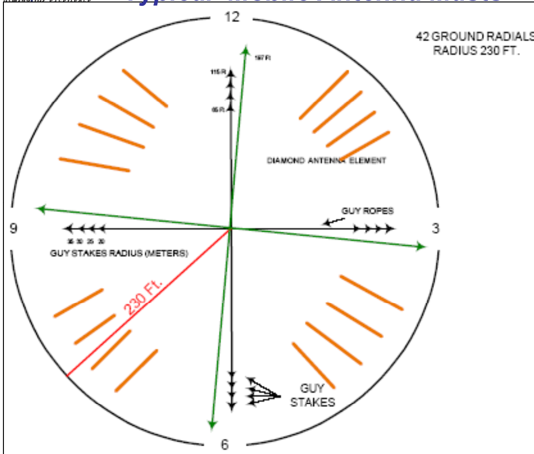
Mast and guy lines & stakes
