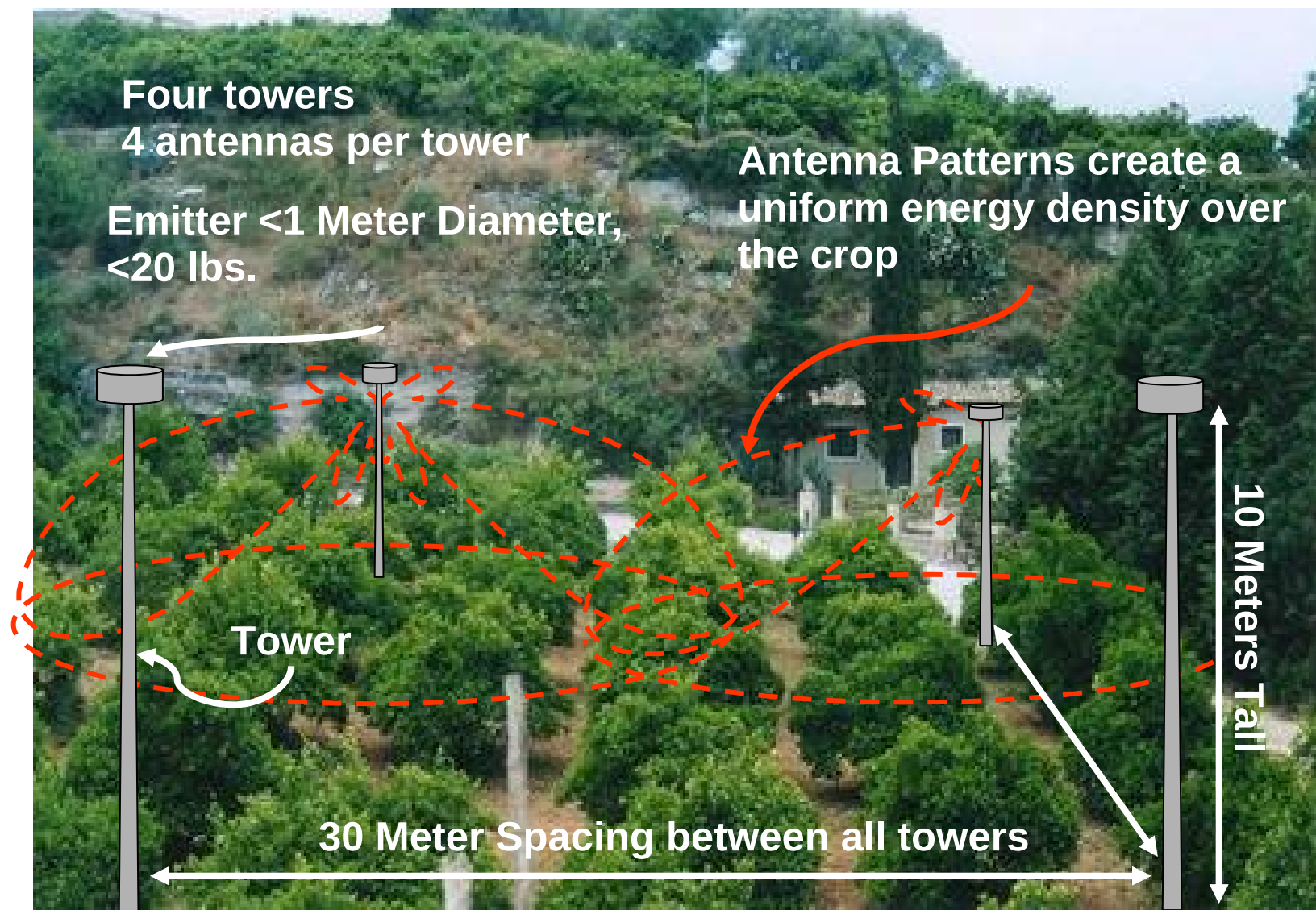
Figure 1. Raytheon's Frost Protection System Test Setup
