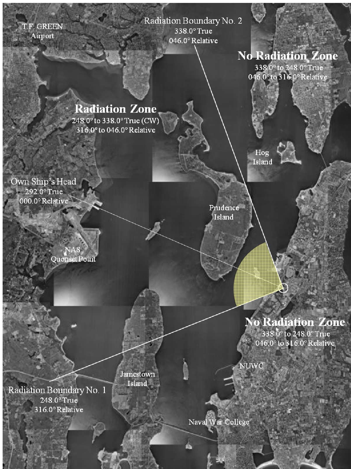
Figure 1. Portsmouth Free Space Radiation Zone (Satellite Image)
