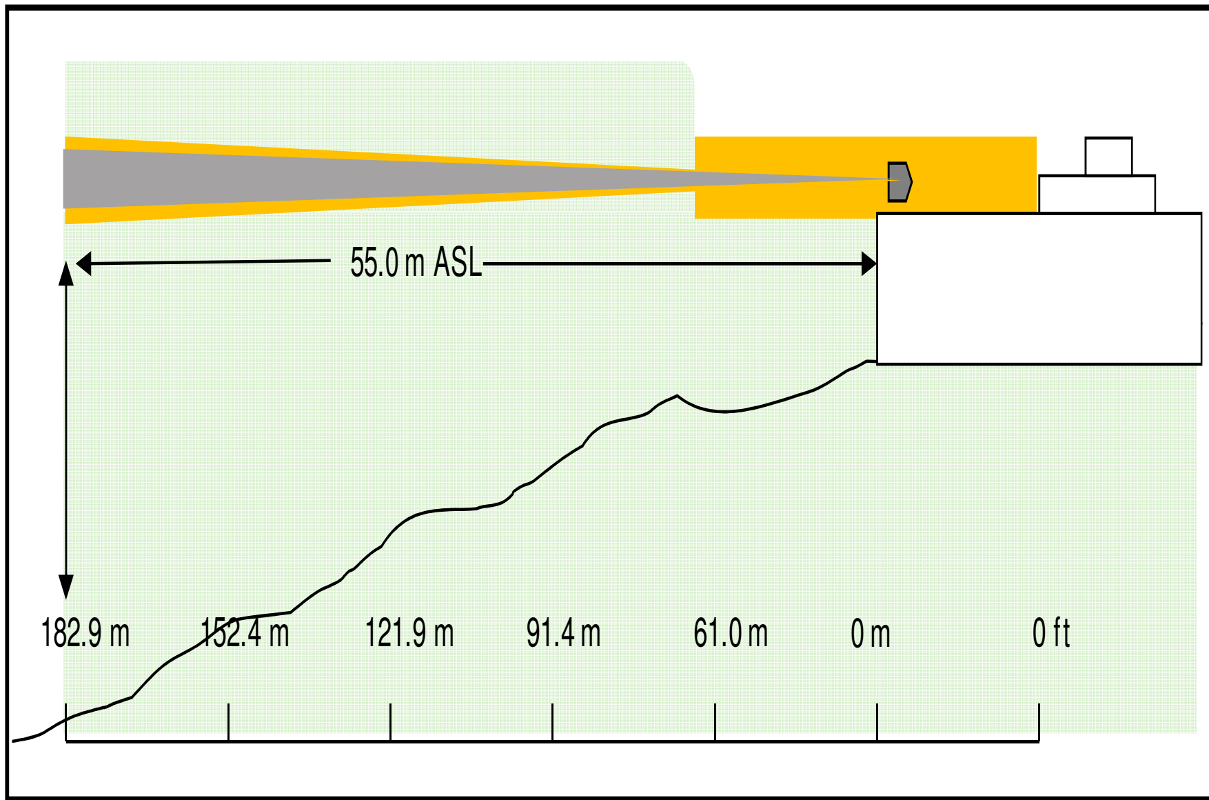
Figure 4. Portsmouth, RI Test Facility. This graphic depicts the location of the radar at the test facility, as well as the intended elevation radiation angle and coverage area. The shaded yellow area defines the Keep-Out Zones (KOZ). Beyond the regions of the KOZ, the power density levels are below limits for uncontrolled environments.
