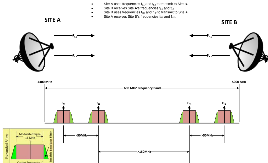
Figure 4 Frequency spacing
