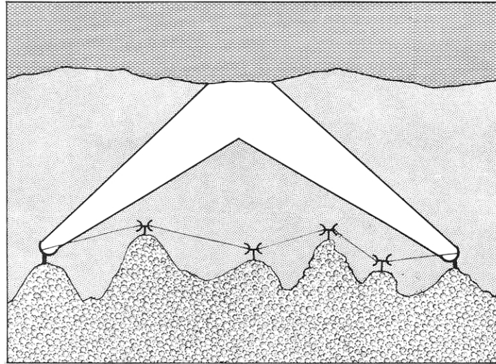
Figure 2 Troposcatter vs line of site
