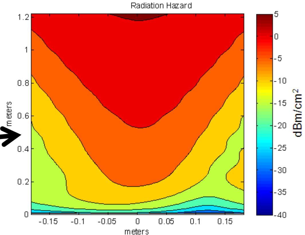
Power Density At Radome End Wall
