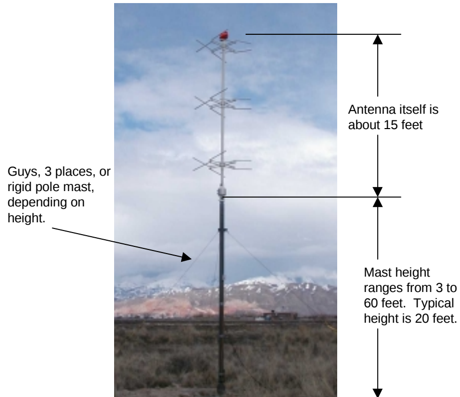
DGPS (LAAS) Ground Station VHF Data Broadcast (VDB) Antenna
