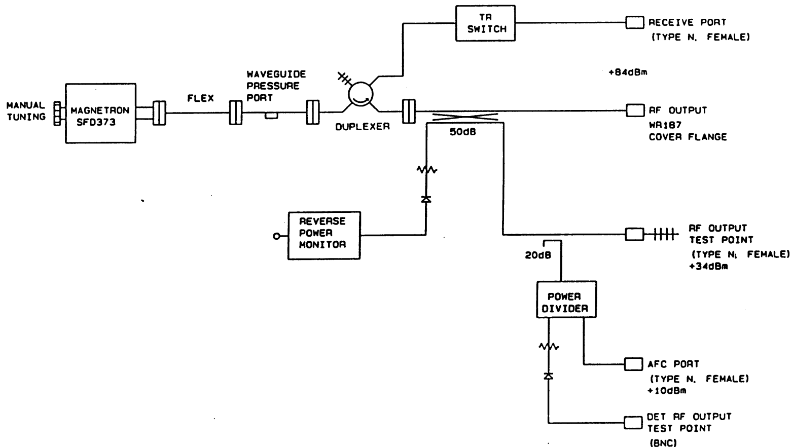
Figure 2c. ASE 541 Magnetron Transmitter RF Block Diagram.
