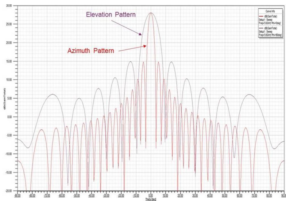
Figure 1 Anticipated Antenna Pattern
