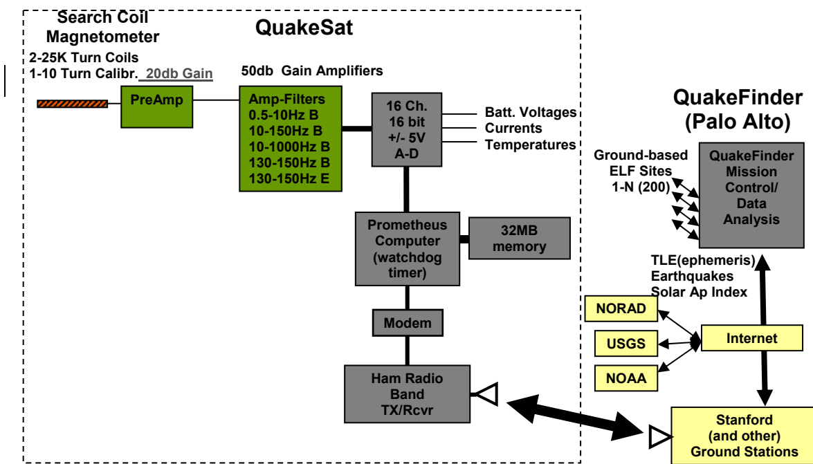
Figure 4: QuakeSat Architecture Block Diagram
