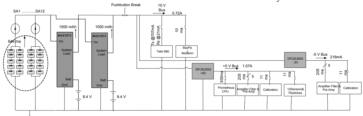
Figure 10: QuakeSat's Electrical Power System
