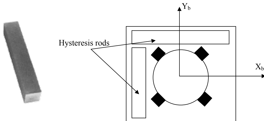
Figure 16: ALNICO 8 HE Magnet and Location in QuakeSat
