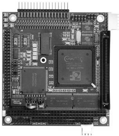
Figure 7: Prometheus PC/104 CPU module
