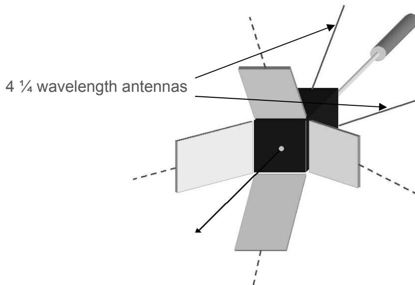
Figure 9: Antenna Placement
