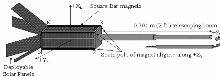
Figure 3: Overview of ELF sensor on Deployable Boom
