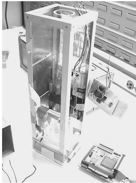
Figure 6. QuakeSat Inner Structure
