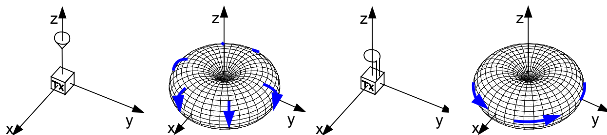
Figure 6a (left): Electric whip antenna and corresponding vertically polarized omni dipole pattern.
