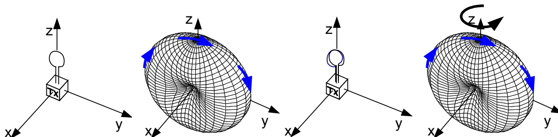
Figure 7a (left): Magnetic loop antenna and corresponding vertically polarized pattern.
