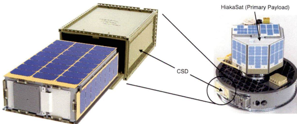
Left: Supernova deploying from Planetary System Corp. Cannisterized Satellite Dispenser (CSD); Right: ORS-4 Integrated Payload Stack, showing location of CSD relative to primary payload (HiakaSat).
