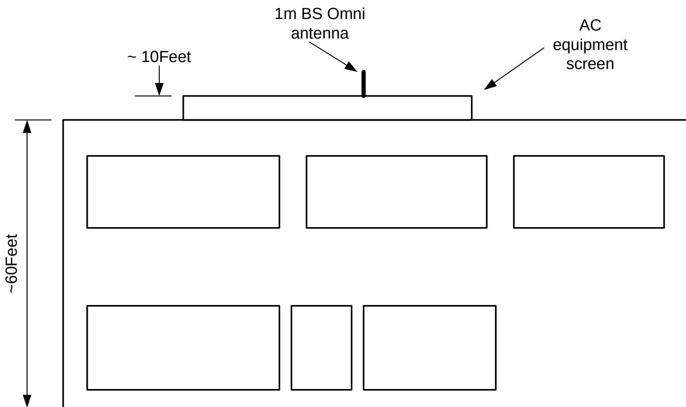
Building Profile View (not to scale)
