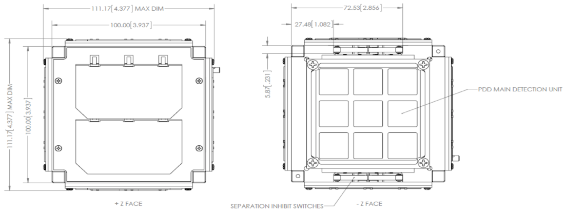
Figure 8: ARMADILLO Width Dimension (mm)
