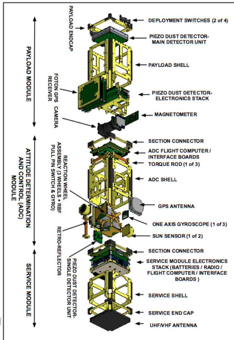
Figure 2: ARMADILLO Expanded View (Not Showing Solar Panels)
