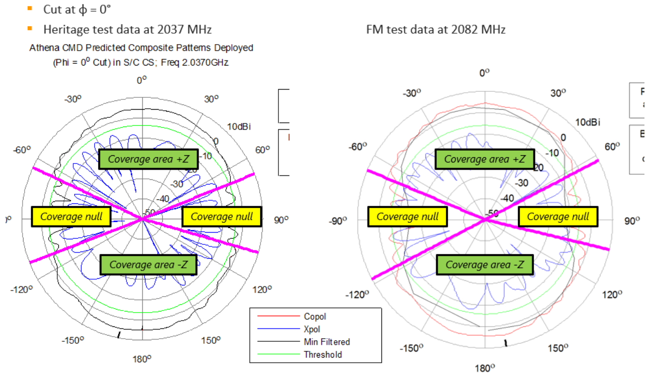
Figure A.6.a-2 TT&C Satellite Antenna Receive Pattern
