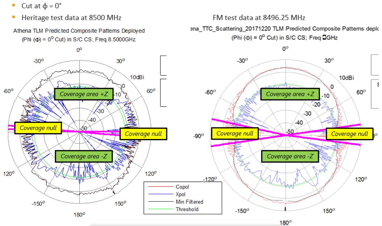
Figure A.6.a-1 TT&C Satellite Antenna Transmit Pattern
