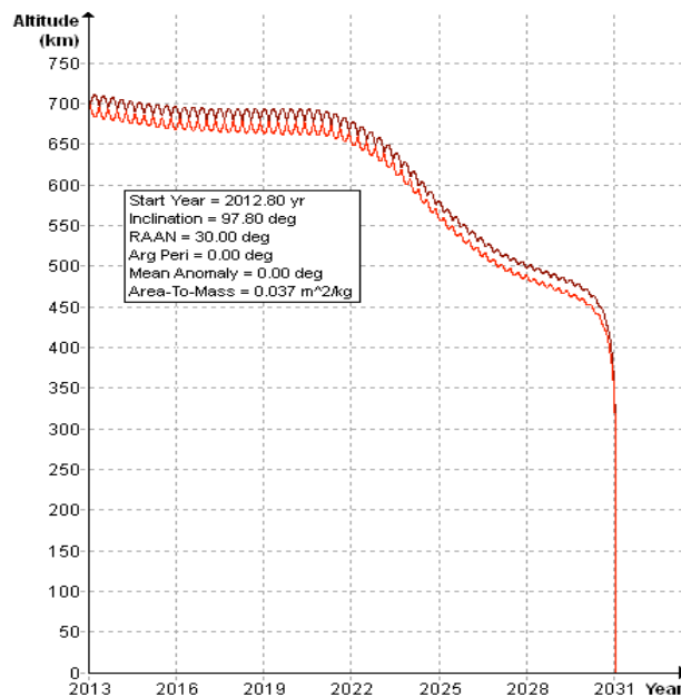
Figure 2 Dove 4 orbit history with apogee (brown) & perigee (red)
