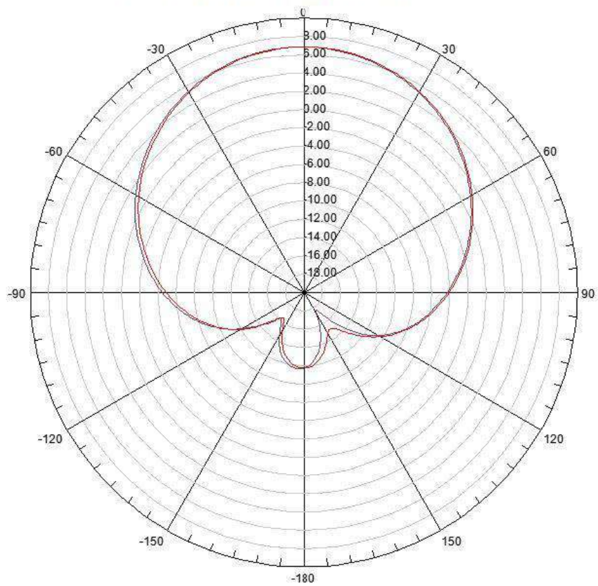
S Band Antenna Radiation Pattern
