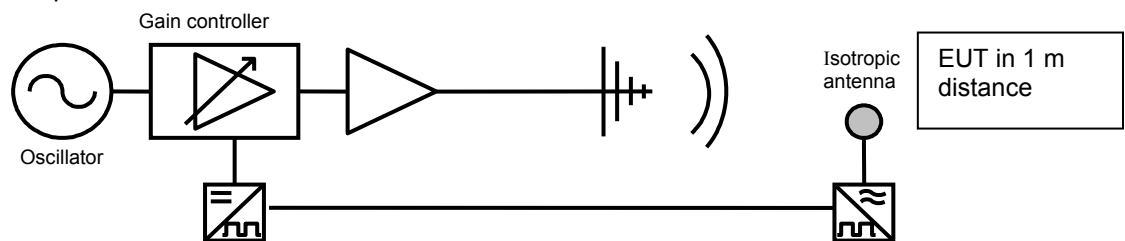
FIGURE 23 : BLOCK DIAGRAM FOR TEST WITH ELECTRIC FIELD CALIBRATION
