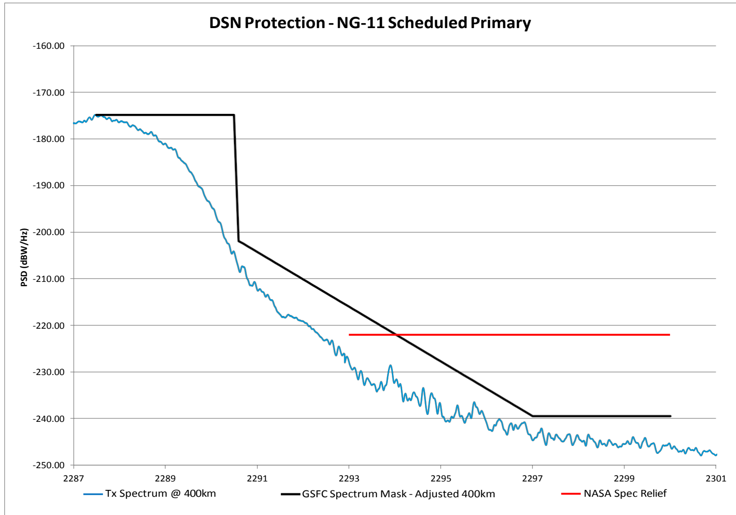
Figure 4 DSN Performance of Emission Designator 6M16G1D with ERP of 6.04 W – Primary Transmitter
