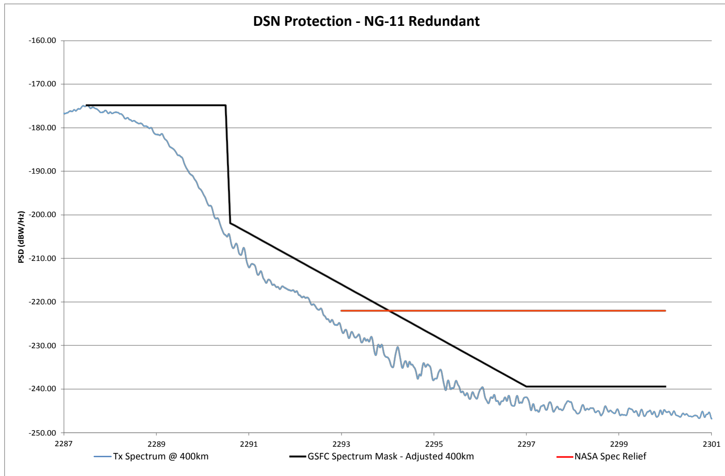
Figure 5 DSN Performance of Emission Designator 6M16G1D with ERP of 6.04 W – Redundant Transmitter
