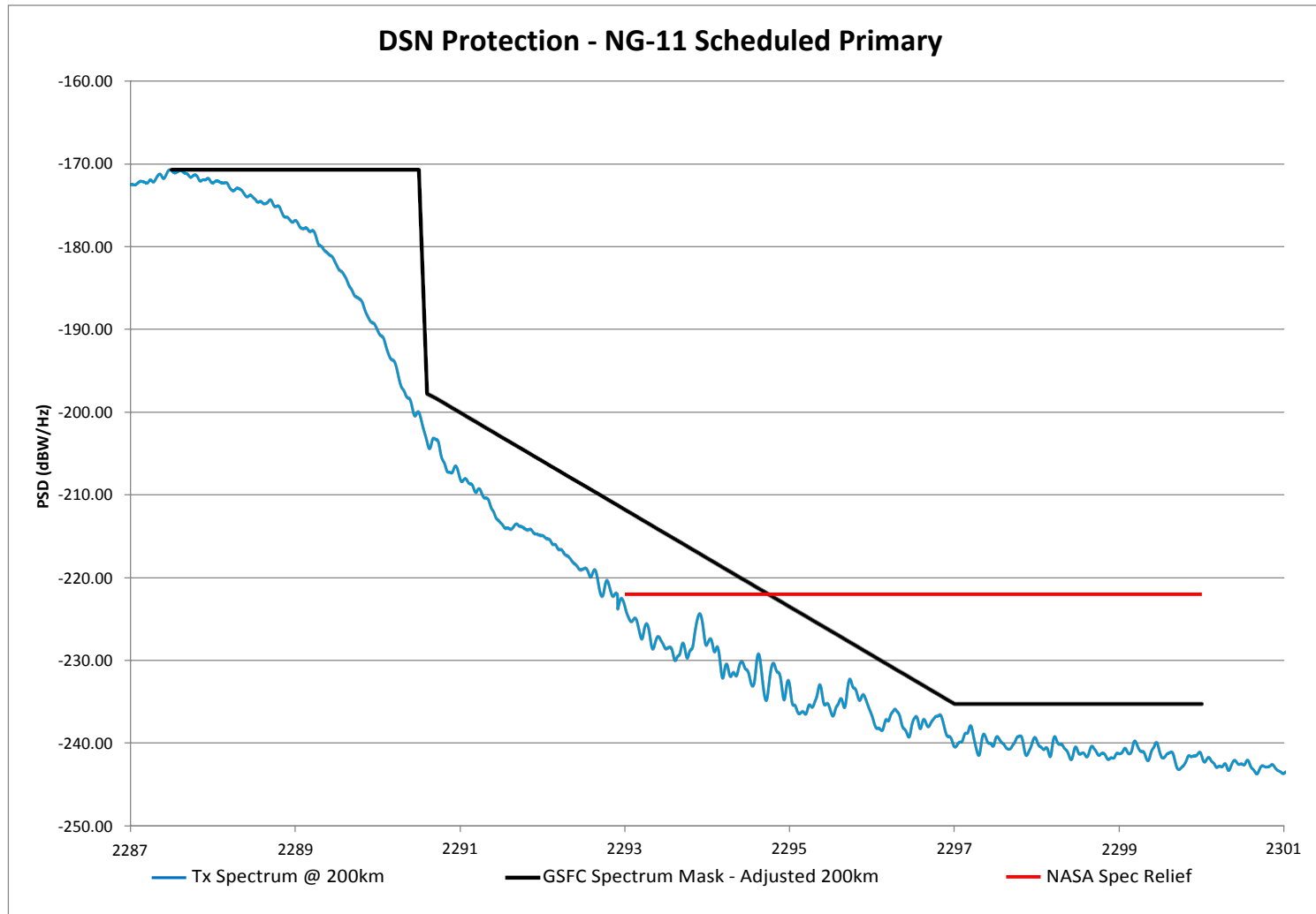
Figure 2 DSN Performance of Emission Designator 6M16G1D with ERP of 4.00 W – Primary Transmitter
