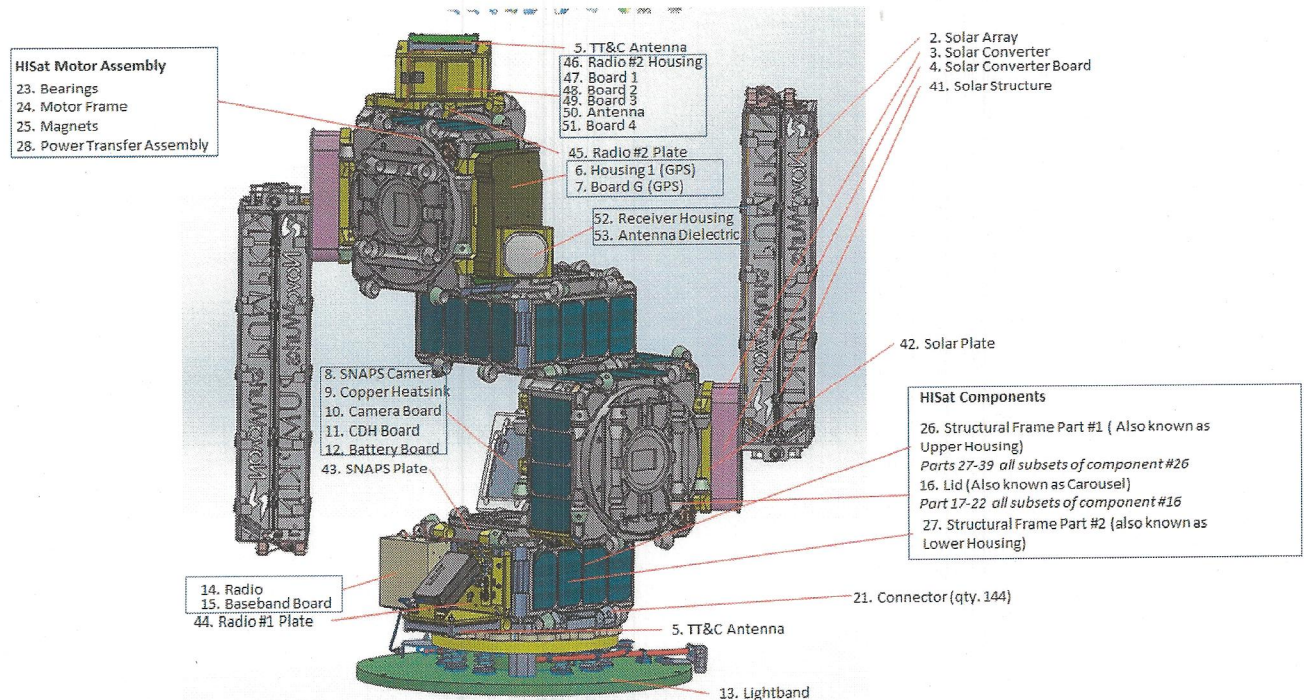
Figure 3 DAS Component Locations
