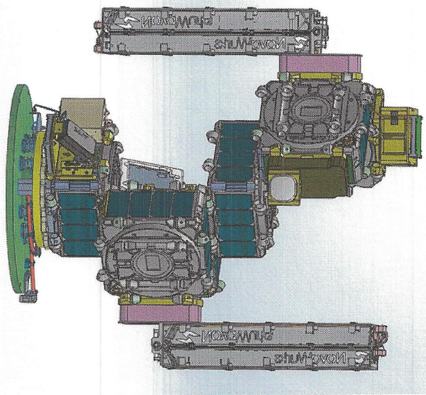
Figure 1 SIMPL – Assembled
