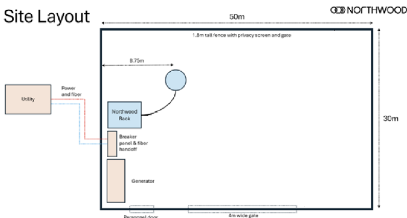
Fig. 1. Layout of Northwood Earth Station Site
