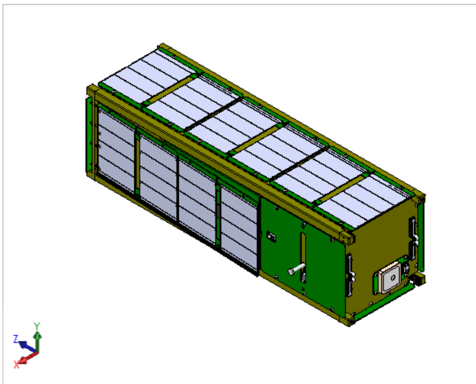
Figure 9: RFTSat with all deployables stowed.
