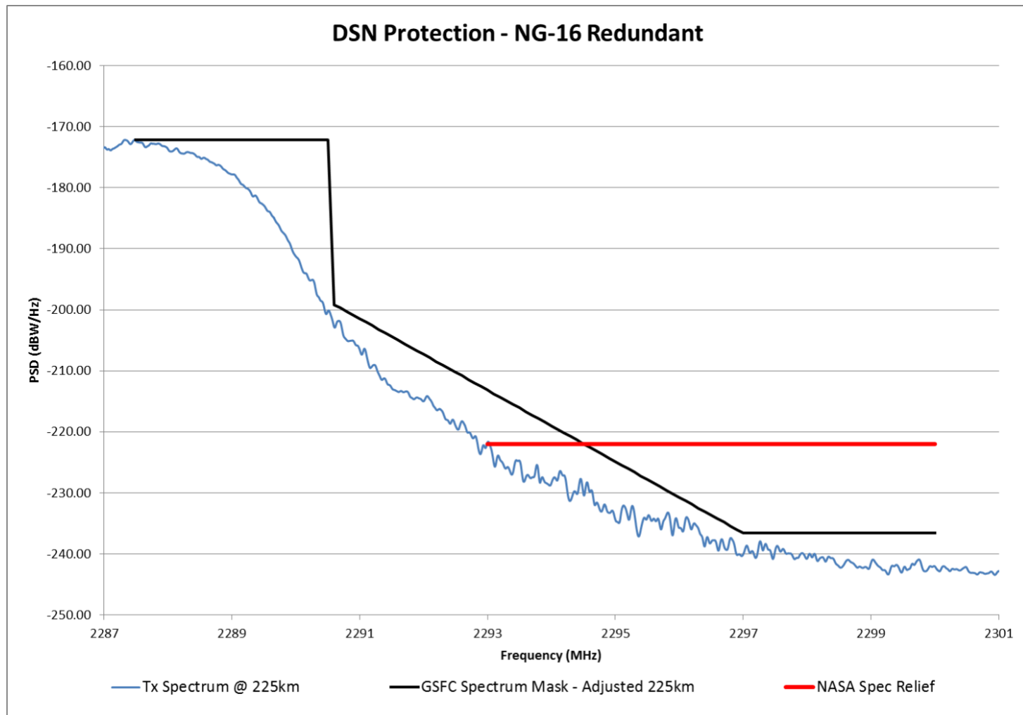
Figure 3. DSN Performance of Emission Designator 6M16G1D with ERP of 3.2 W – Redundant Transmitter
