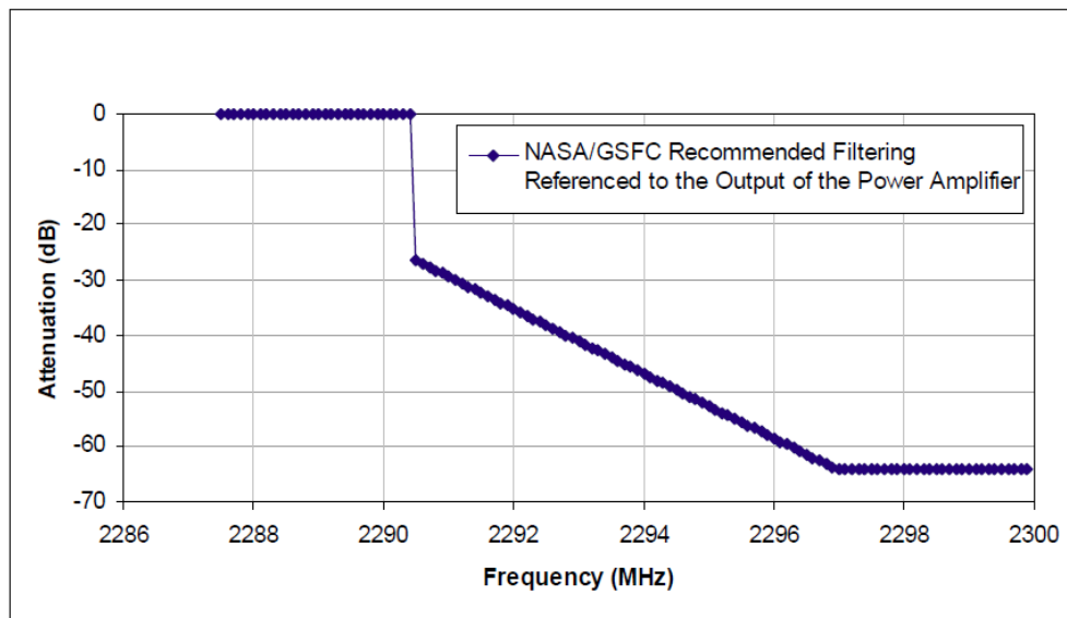
Figure 1. Spectral Output for NASA/GSFC Recommended Filtering Referenced to Output of Power Amplifier (from 450-SNUG Figure D-6)
