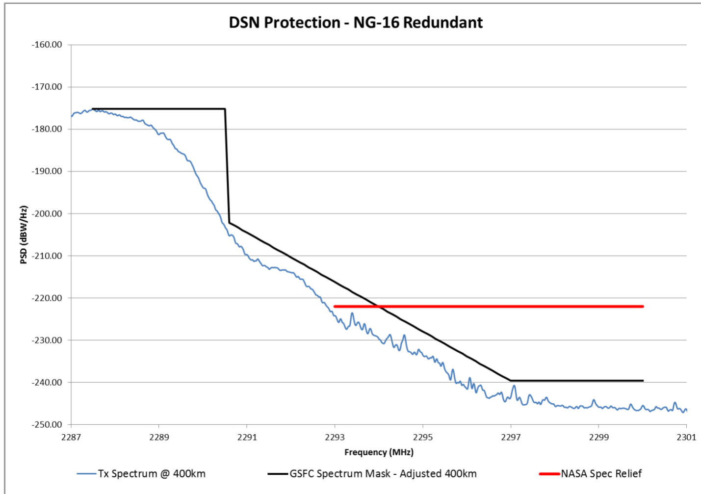
Figure 5. DSN Performance of Emission Designator 6M16G1D with ERP of 5.1 W – Redundant Transmitter
