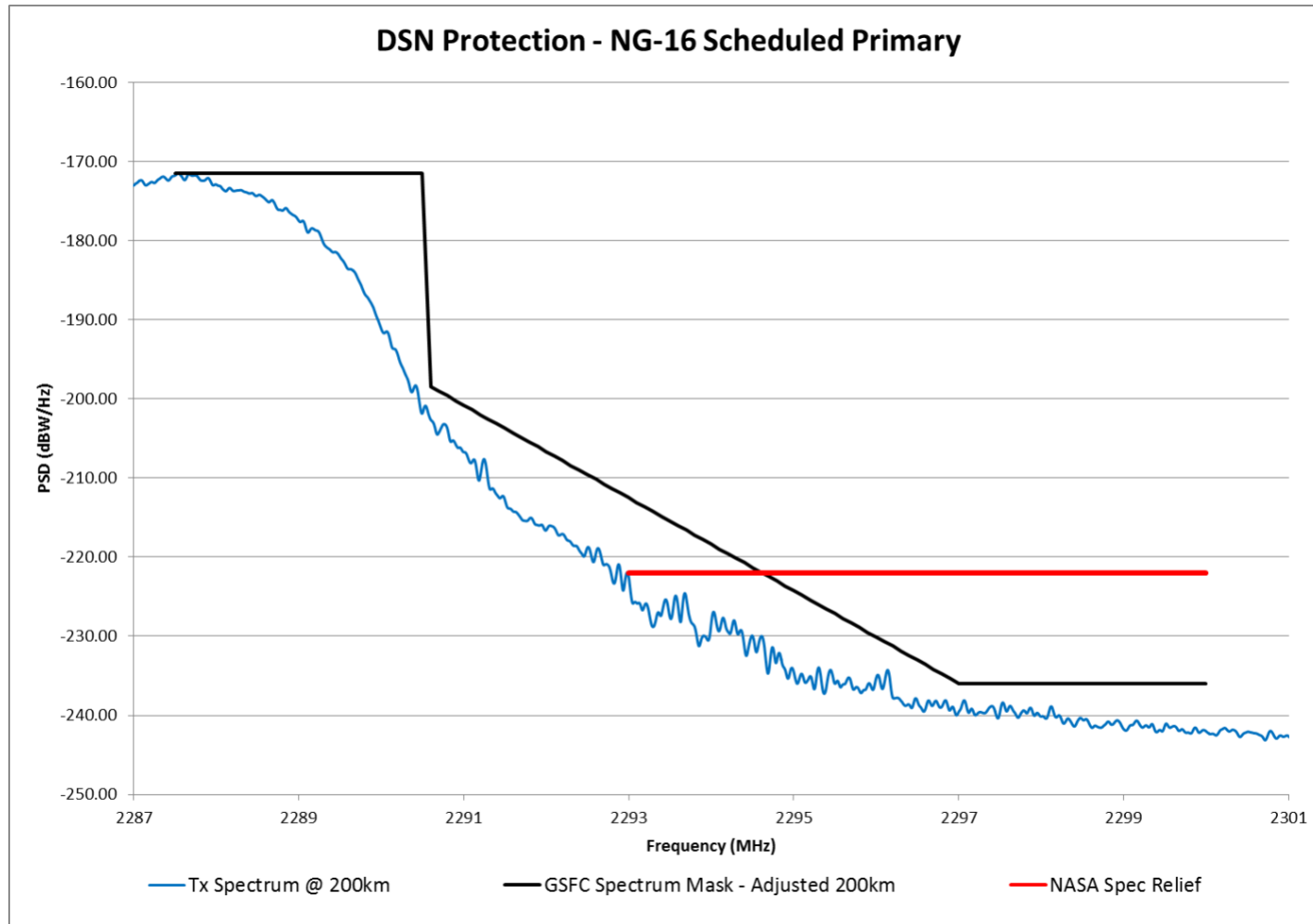
Figure 2. DSN Performance of Emission Designator 6M16G1D with ERP of 3.2 W – Primary Transmitter
