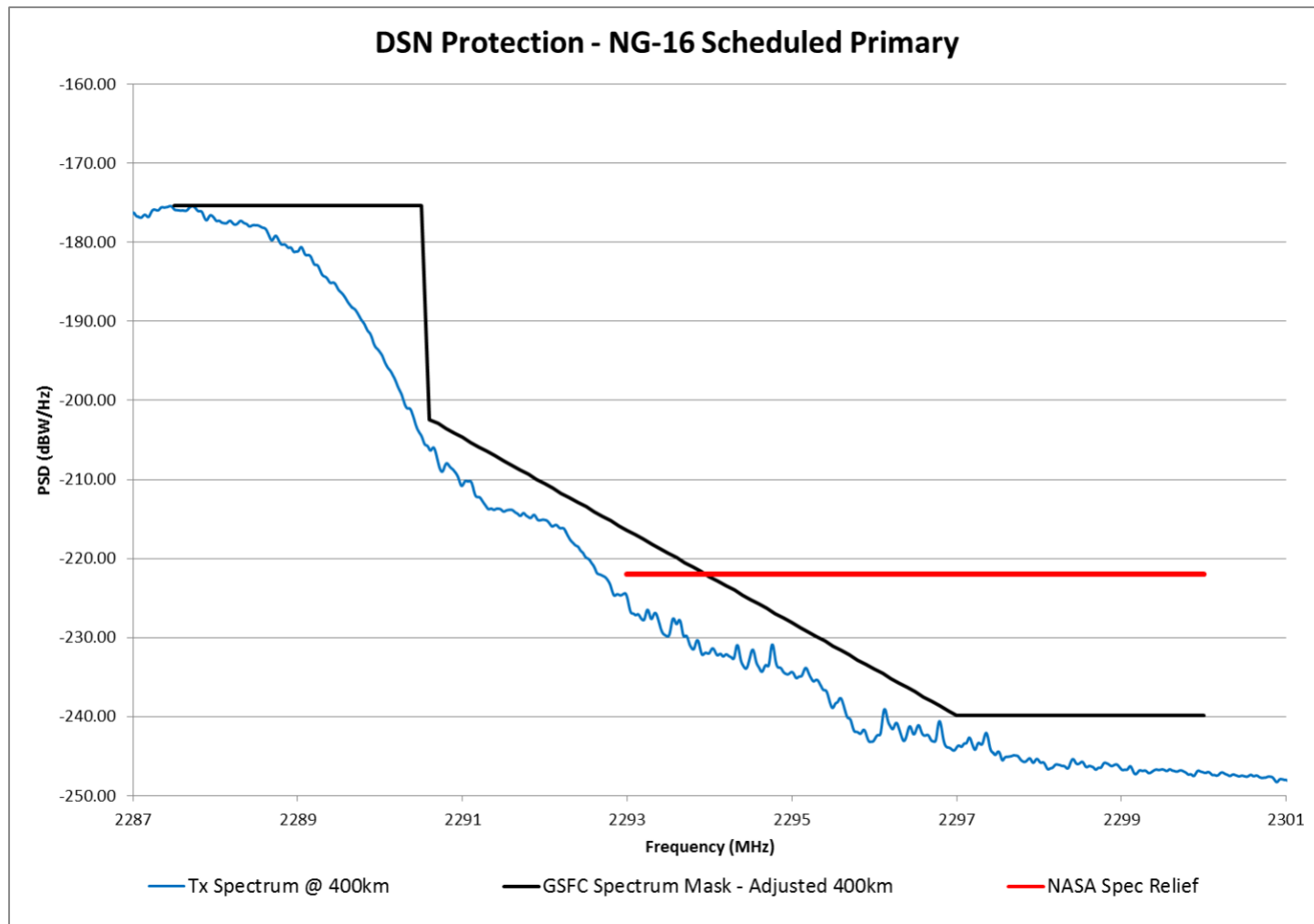
Figure 4. DSN Performance of Emission Designator 6M16G1D with ERP of 5.1 W – Primary Transmitter
