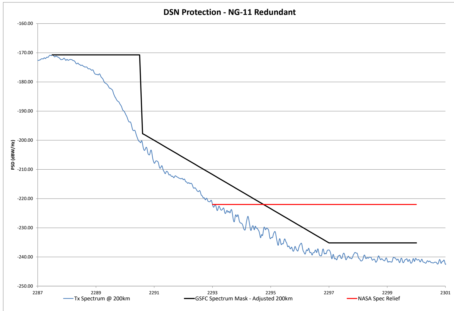
Figure 3 DSN Performance of Emission Designator 6M16G1D with ERP of 4.00 W – Redundant Transmitter
