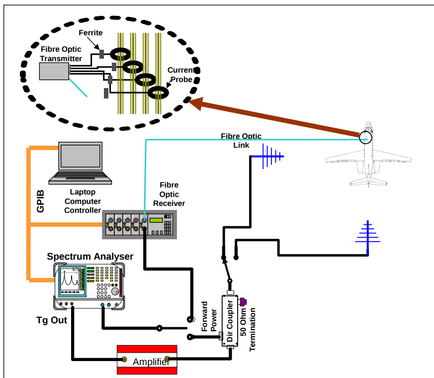
Figure 3 - LLSC Test Set-up Schematic
