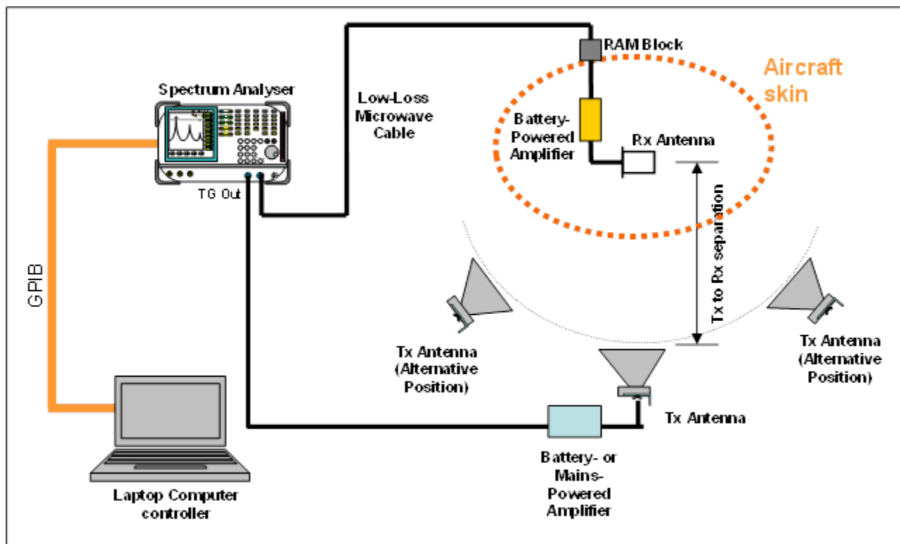
Figure 7 - LLSF Test Set-up Schematic
