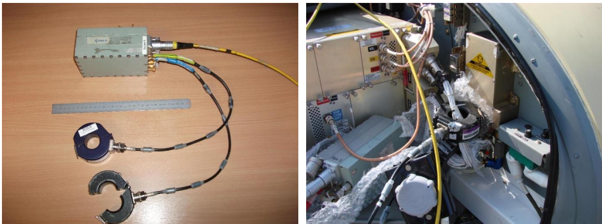
Figure 1 - LLSC Current Probes and FOL
