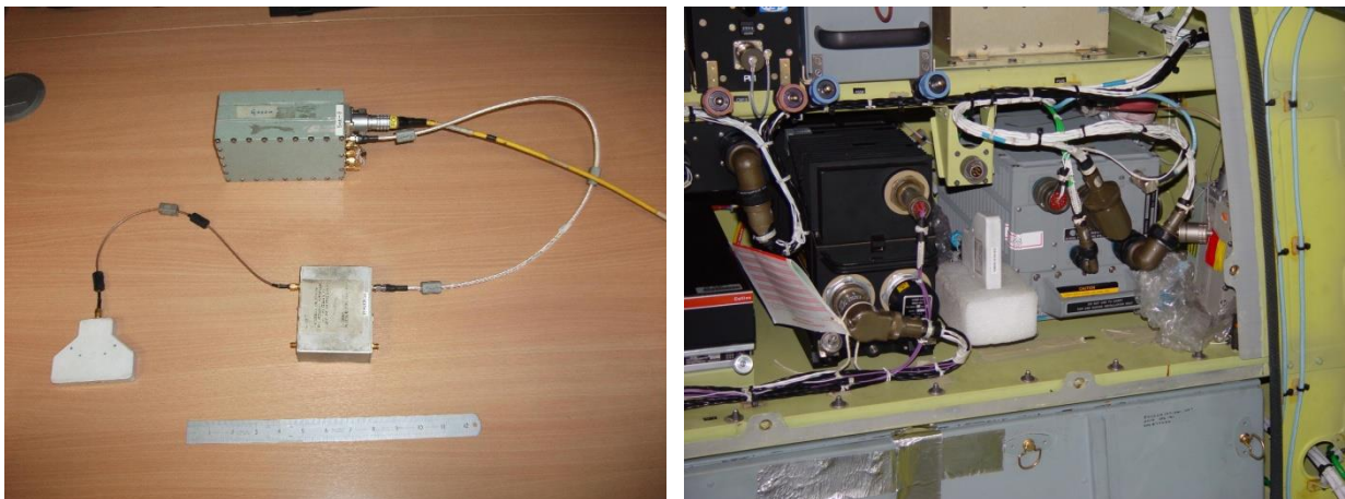
Figure 4 - LLSF Receive Antenna (Below 1 GHz) and FOL
