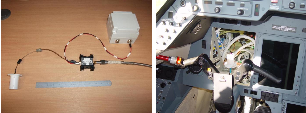
Figure 5 - LLSF Receive Antenna (Above 1 GHz) & Battery-powered Pre-amplifier
