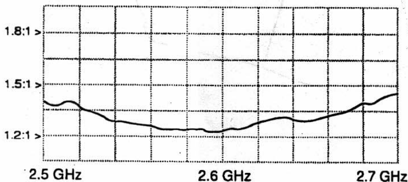
Typical VSWR
