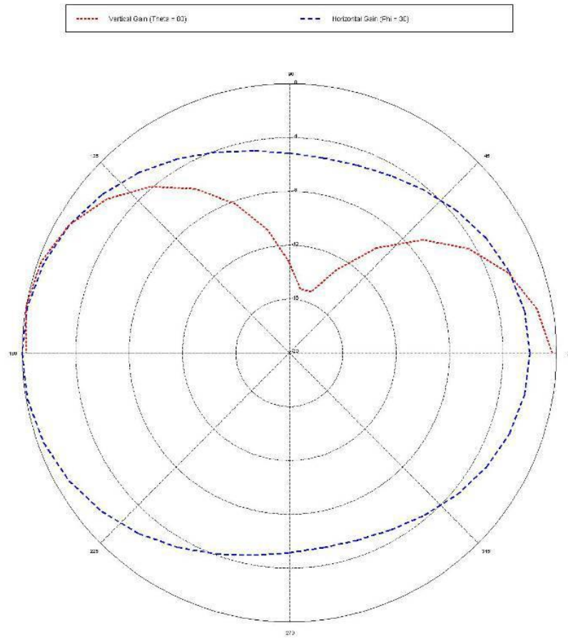
Dipole Antenna on 30 Structure
