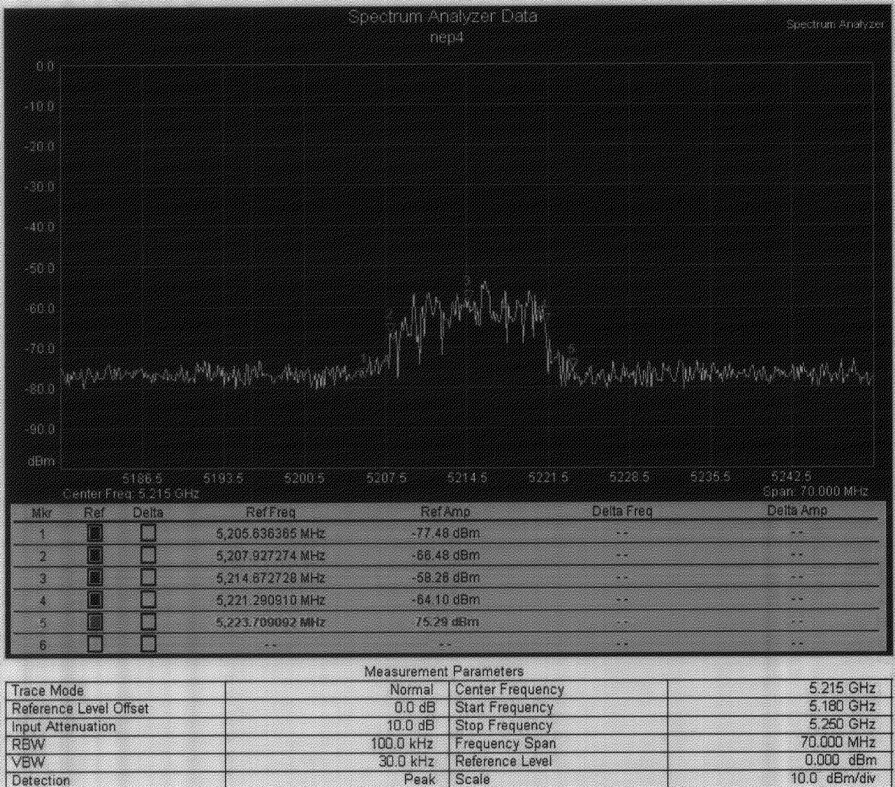
Figure 4 – NEP4, 5.205 – 5.223 GHz.
