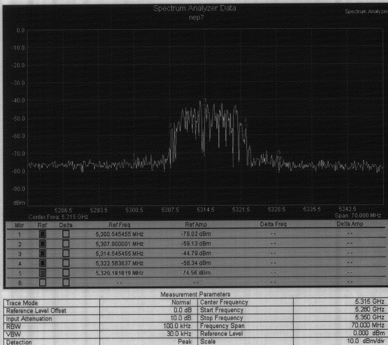
Figure 9 – NEP7, 5.300 – 5.329 GHz.
