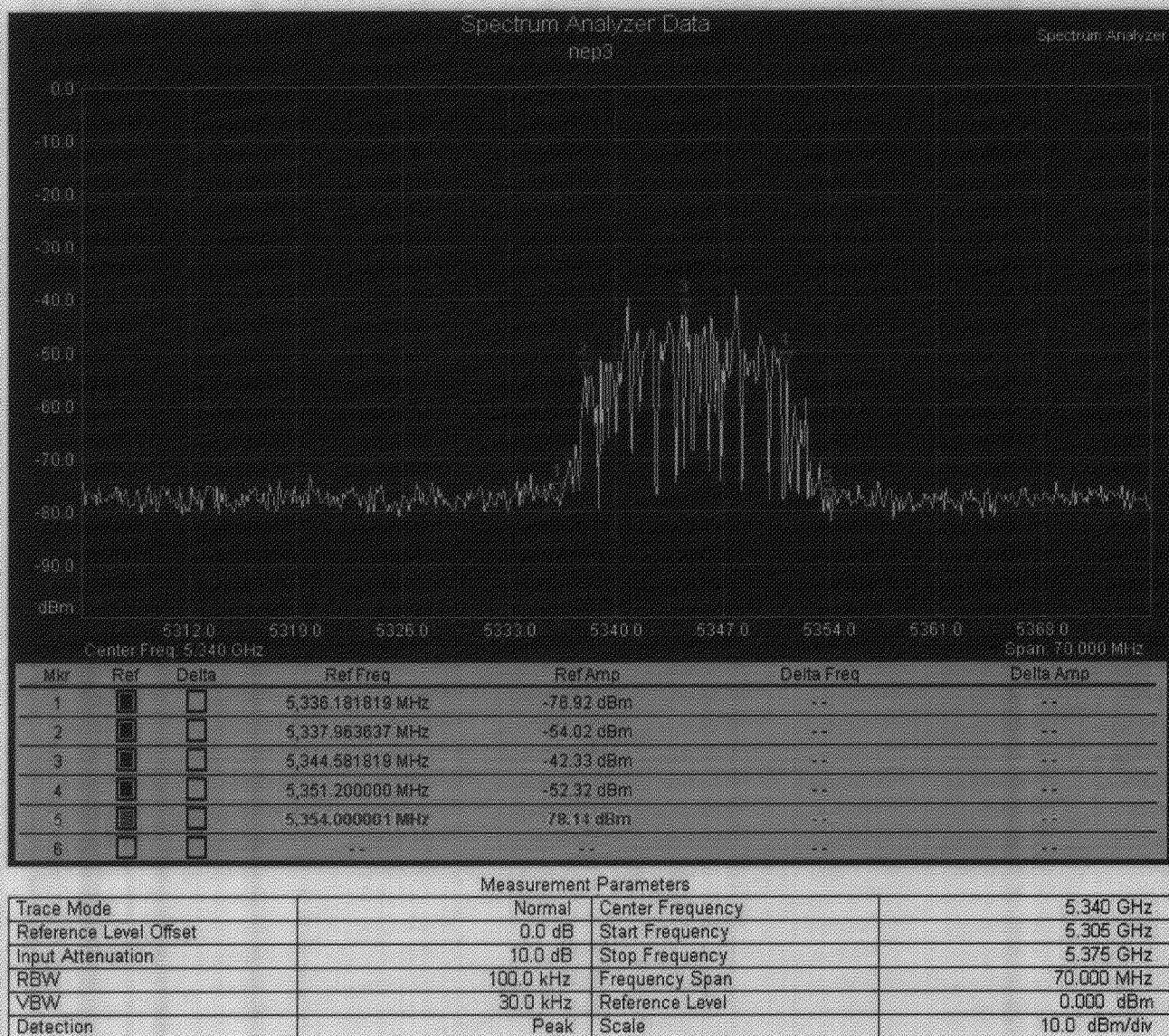
Figure 3 – NEP3, 5.336 – 5.354 GHz.
