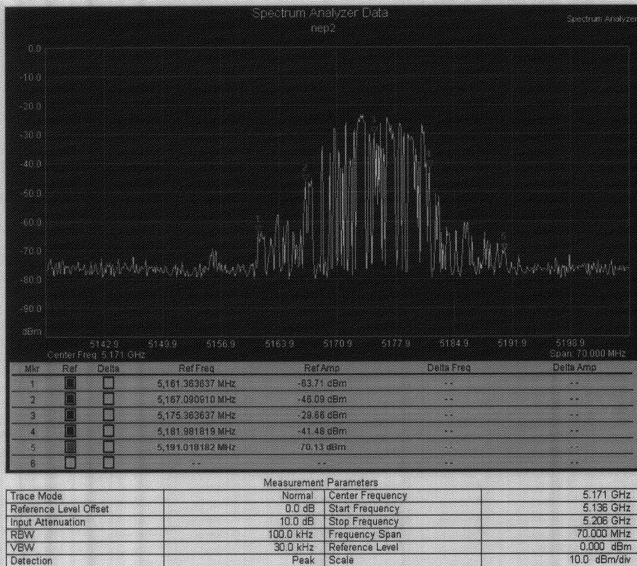
Figure 2- NEP2, 5.161 – 5.191 GHz.
