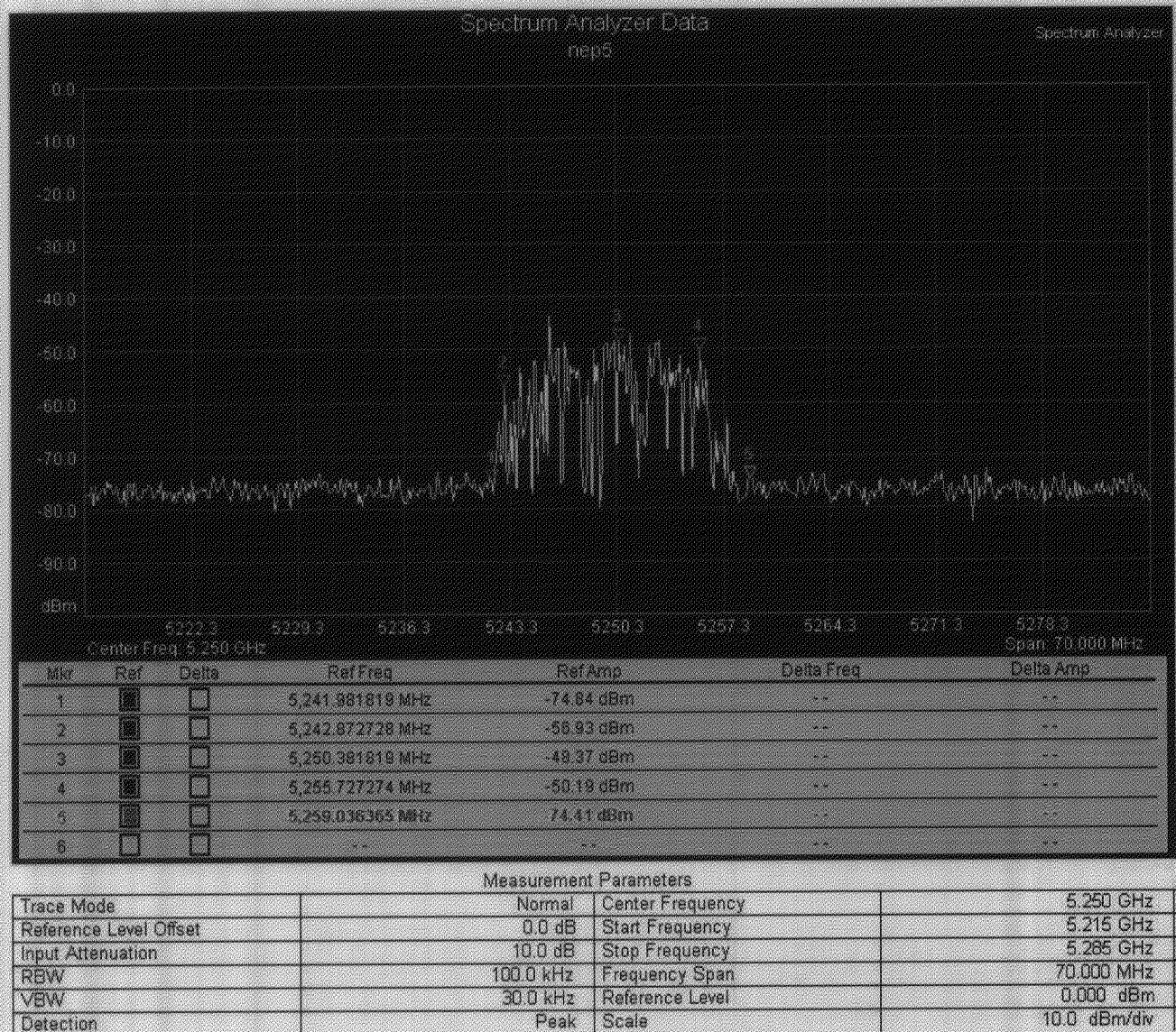
Figure 6 – NEP5, 5.241 – 5.259 GHz.
