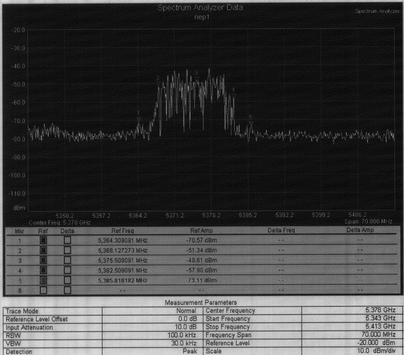
Figure 1 – NEP1, 5.364 – 5.385 GHz.
