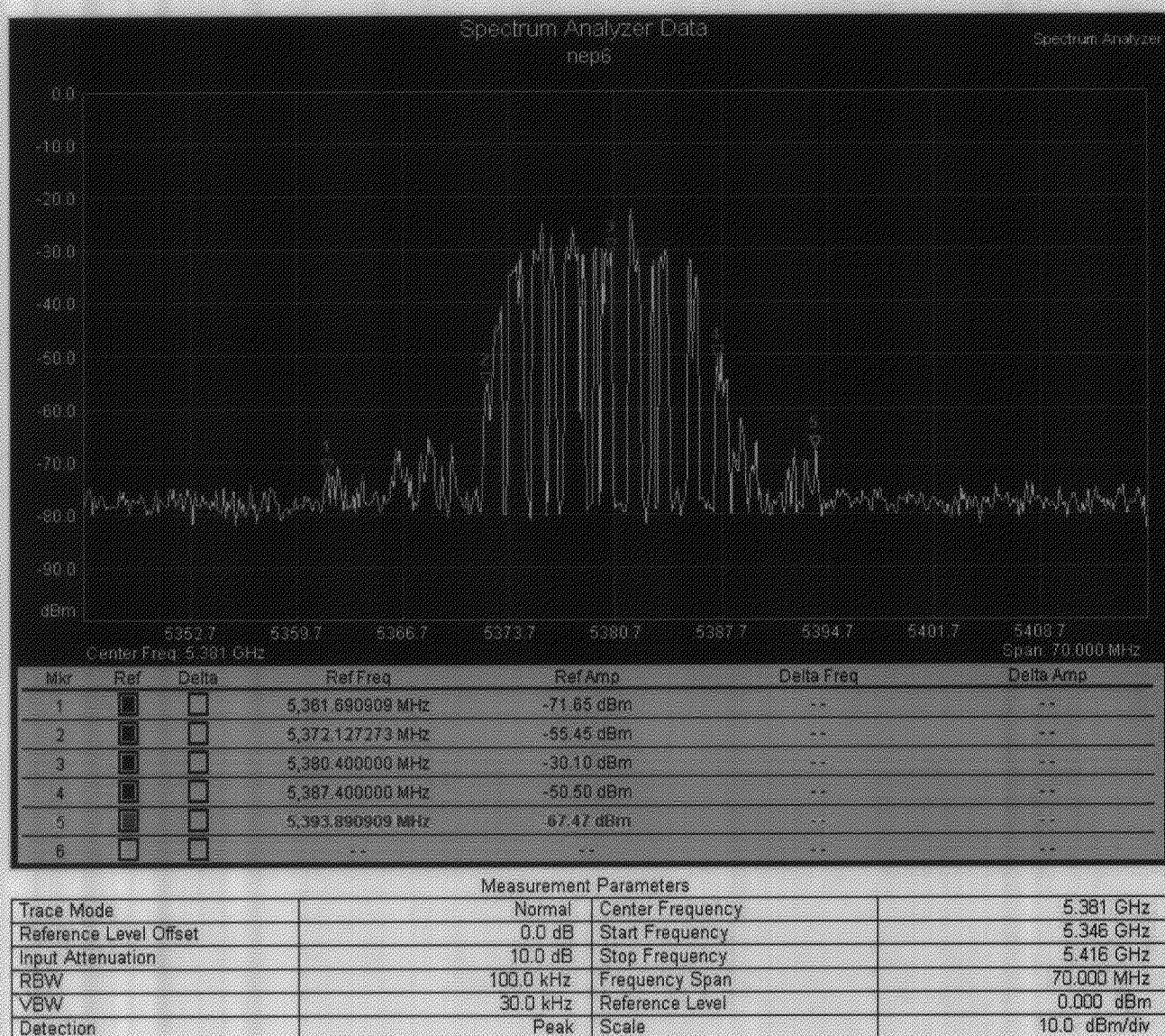
Figure 8 – NEP6, 5.361 – 5.393 GHz.
