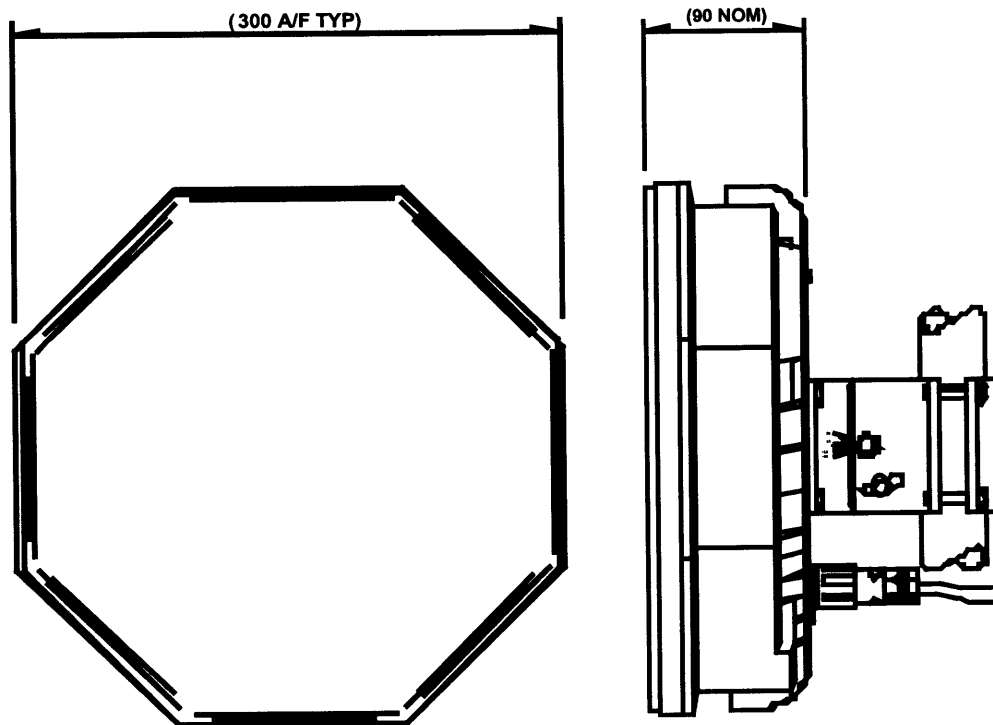
Figure 3 - PROXIMITY-I™ RTU
