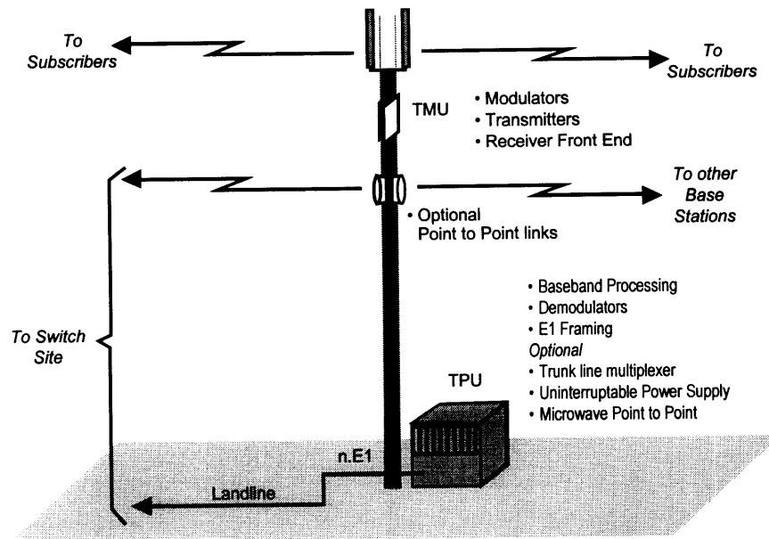
Figure 2 - PROXIMITY-I™ Basestation
