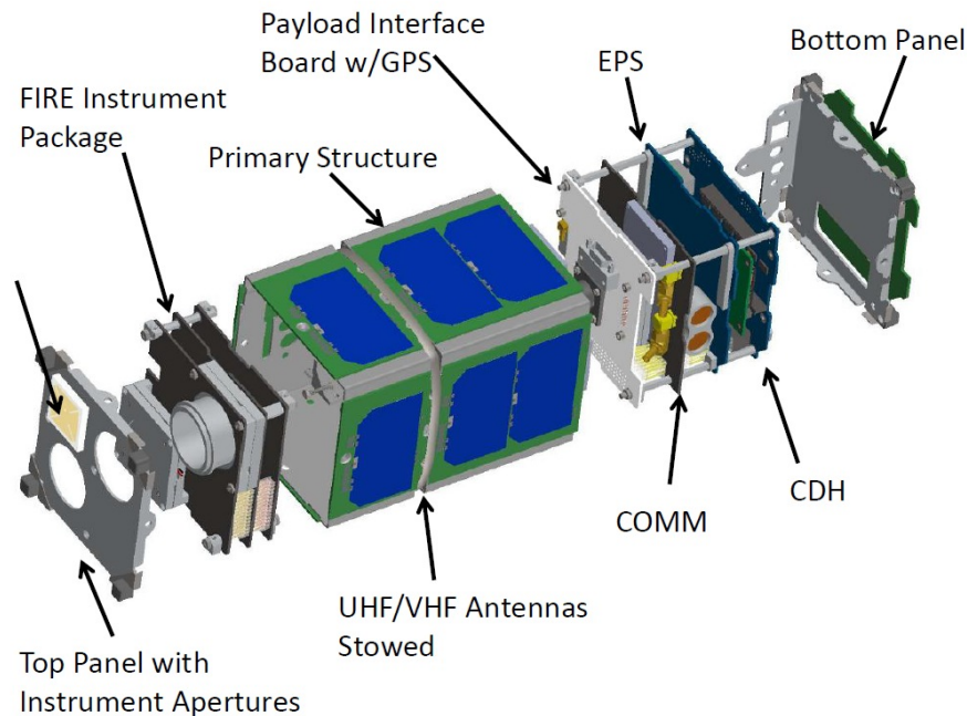
Figure 2: FIREBIRD Expanded View
