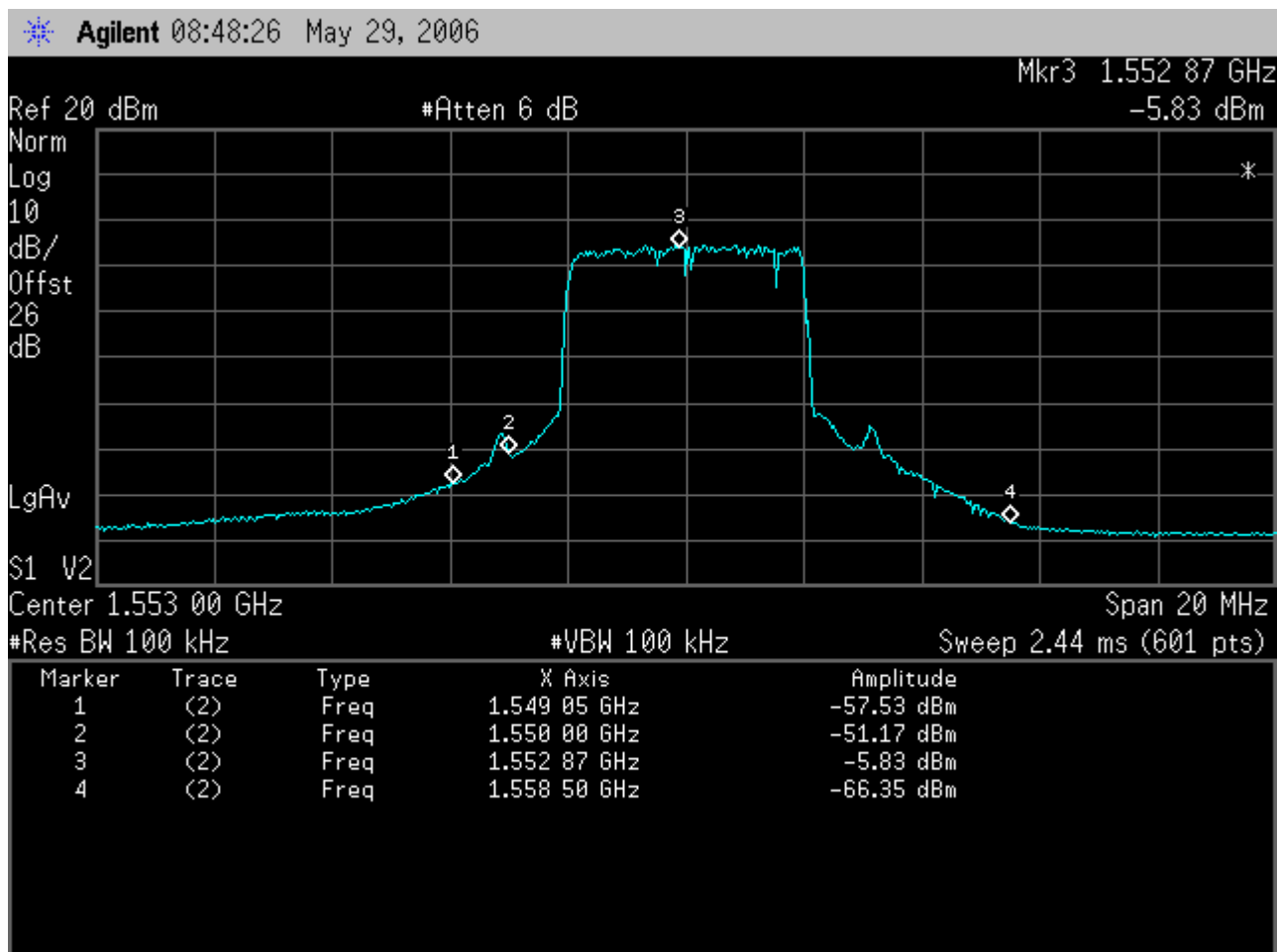
Figure 1: Carrier Spectrum Mask Measurements
