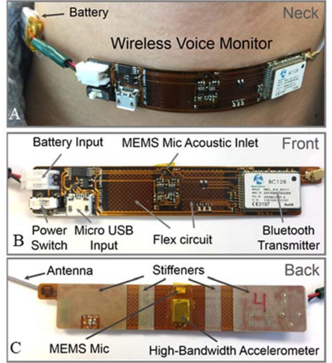
Figure 2. Wireless voice monitor, showing (A) transmitter circuitry on the anterior neck surface, (B) components on the front layer of the flexible circuit, and (C) components on the back layer.
