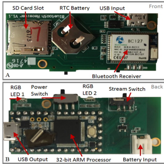
Figure 3. Wireless voice monitor's receiver. Components on the (A) front layer and (B) back layer of the circuit board.
