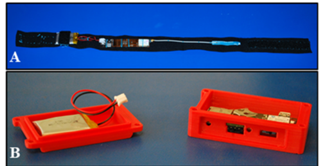
Figure 5. Packaged wireless voice monitor. (A) transmitter components sewn on fabric neck strap and (B) enclosed receiver.
