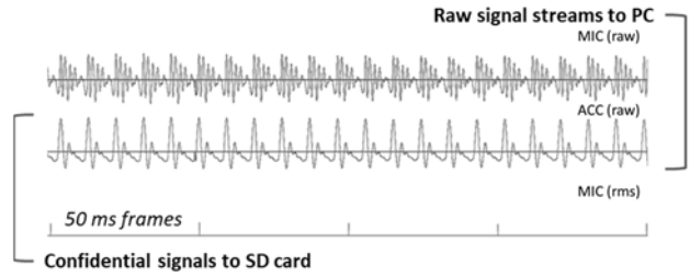
Figure 4. Sensor signals being transferred throughout the system. Laboratory data include raw ACC and MIC signals, whereas ambulatory recordings save data channels to preserve confidentiality (raw ACC and averaged MIC rms signals).
