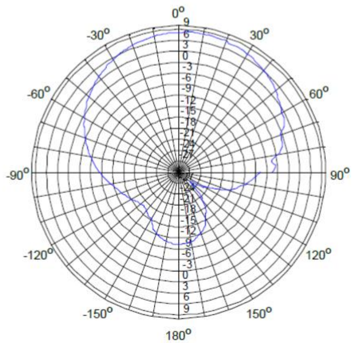
Transmit Pattern (typical), 7.3 dB Gain Average
