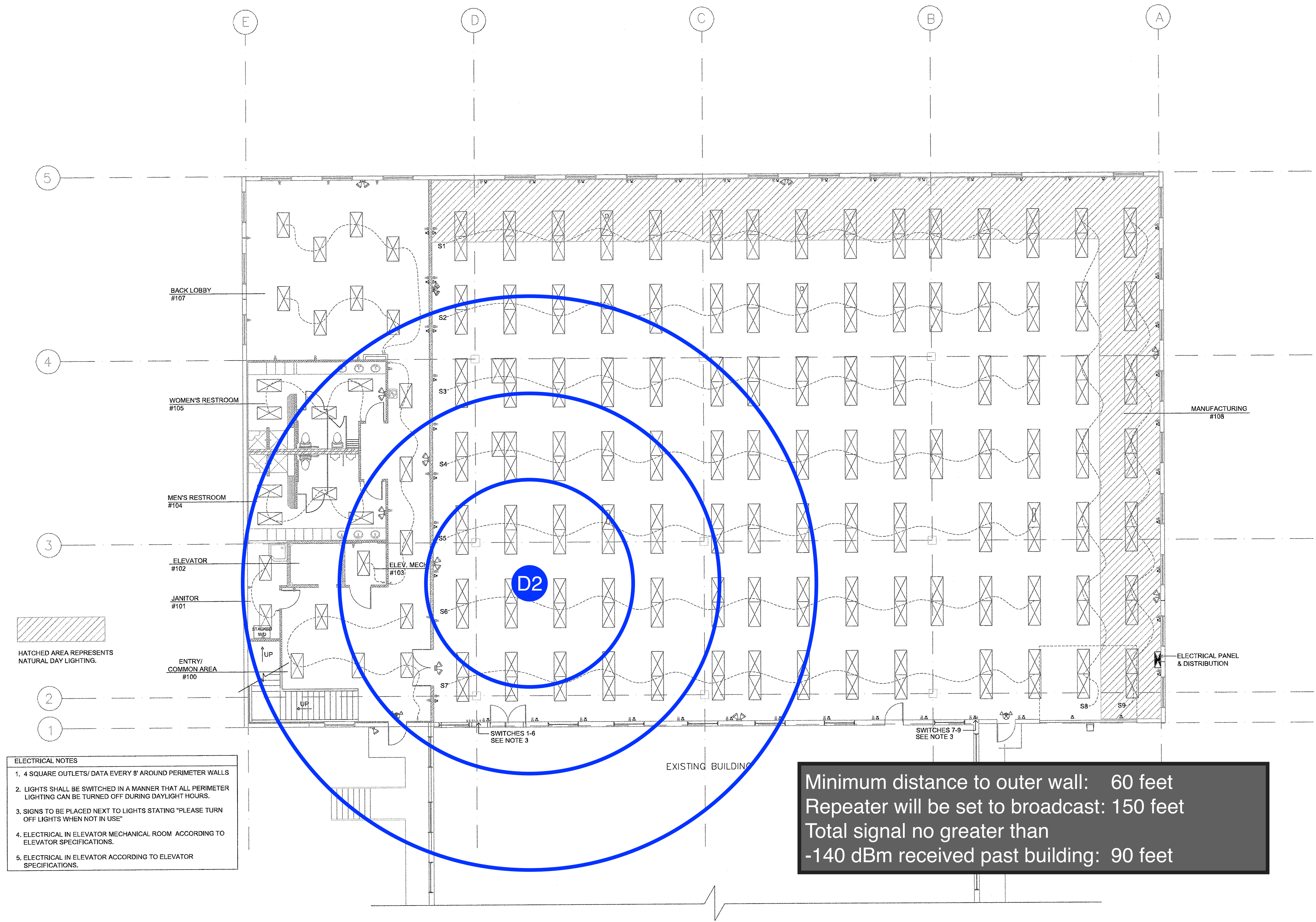
1 FIRST FLOOR ELECTRICAL PLAN SCALE 1/8" = 1'-0"
