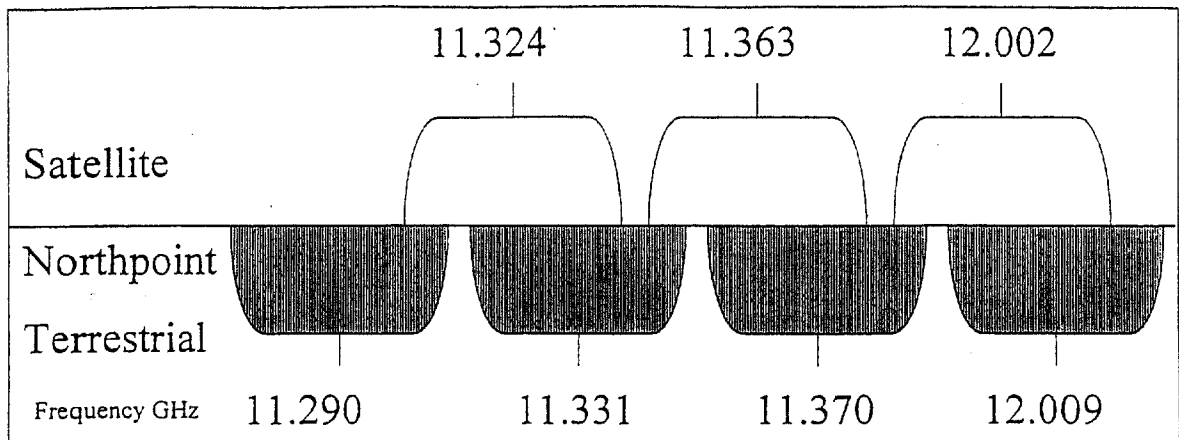
Figure 2: Proper use of frequency offset mitigation technique
