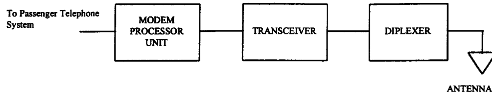
Figure 2 Terrestrial Flight Telephone System Aircraft Station Block Diagram
