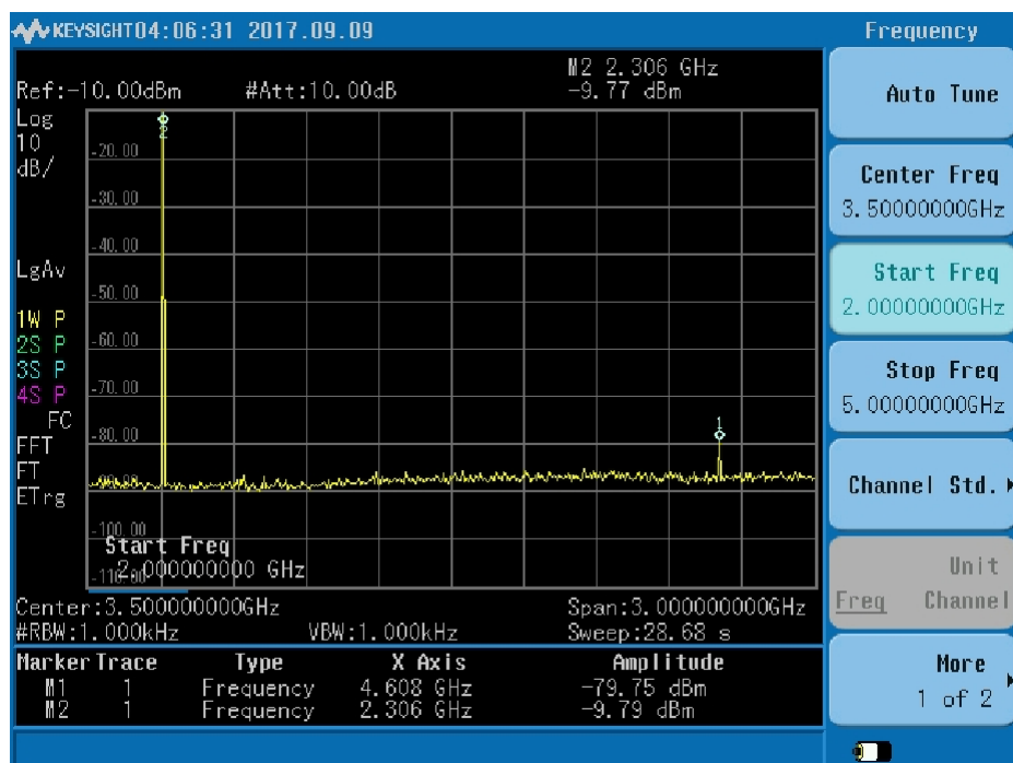
Figure 2 (Harmonic Measurement)
