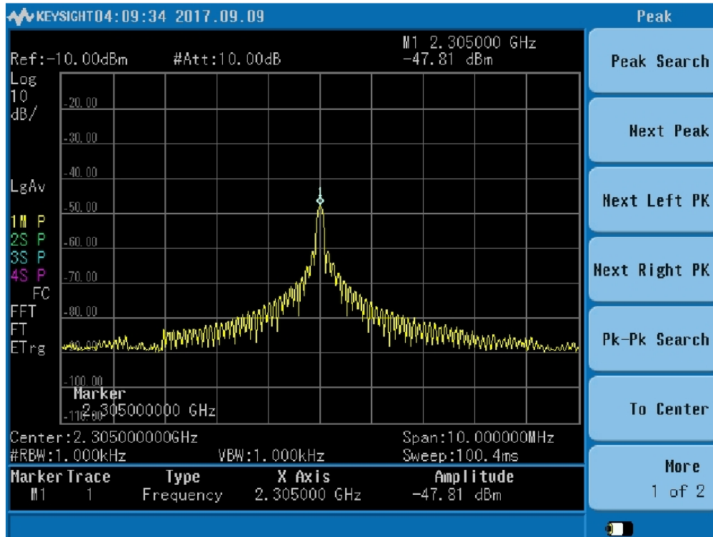
Figure 3 (Bandwidth Measurement)
