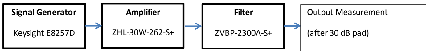
Figure 1 (Test Setup)
