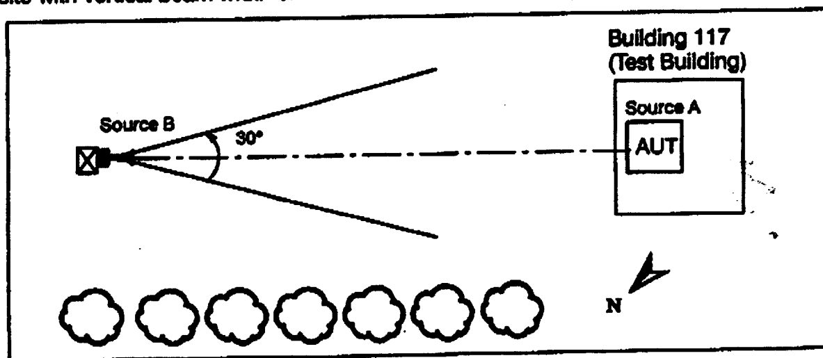
Figure 2: Top View of the Antenna Test Facility
