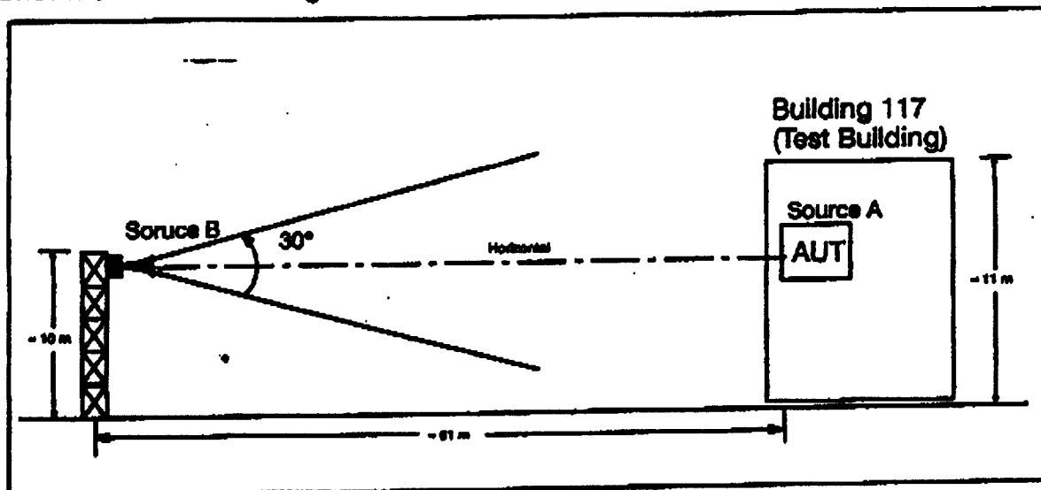
Figure 1: Side View of the Antenna Test Facility
