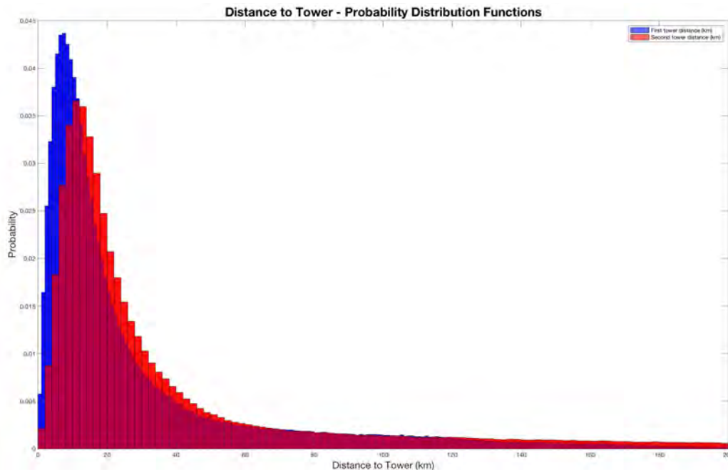
Figure 20 - Probability distribution function (PDF) of the distance to the first and second nearest tower for any location in the US per the Monte Carlo simulation model
