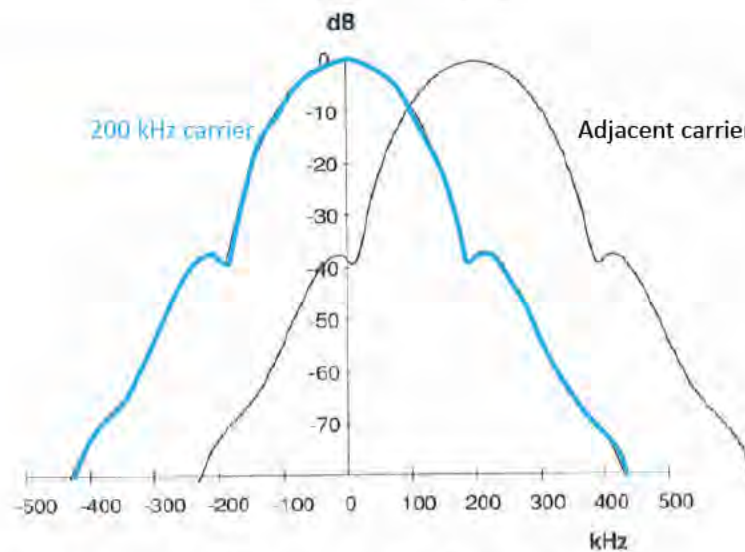
[REDACTED] GSM spectrum showing ACI Level in a 200 kHz channel
