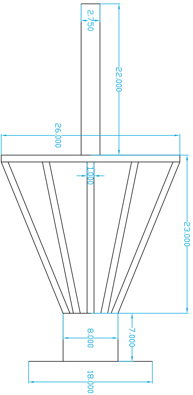
ANT260K (95MHz-3Ghz)
