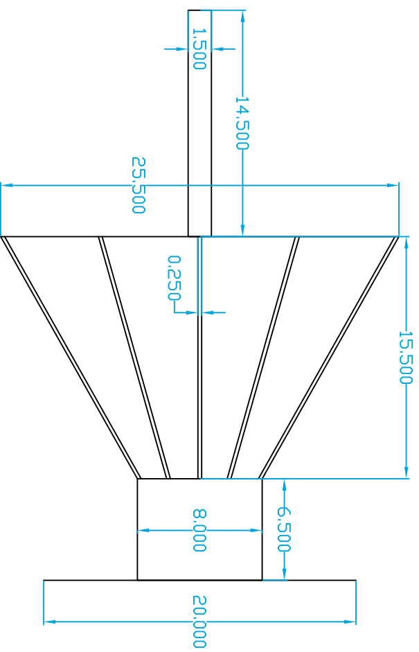
ANT280S (118MHz-3Ghz)
