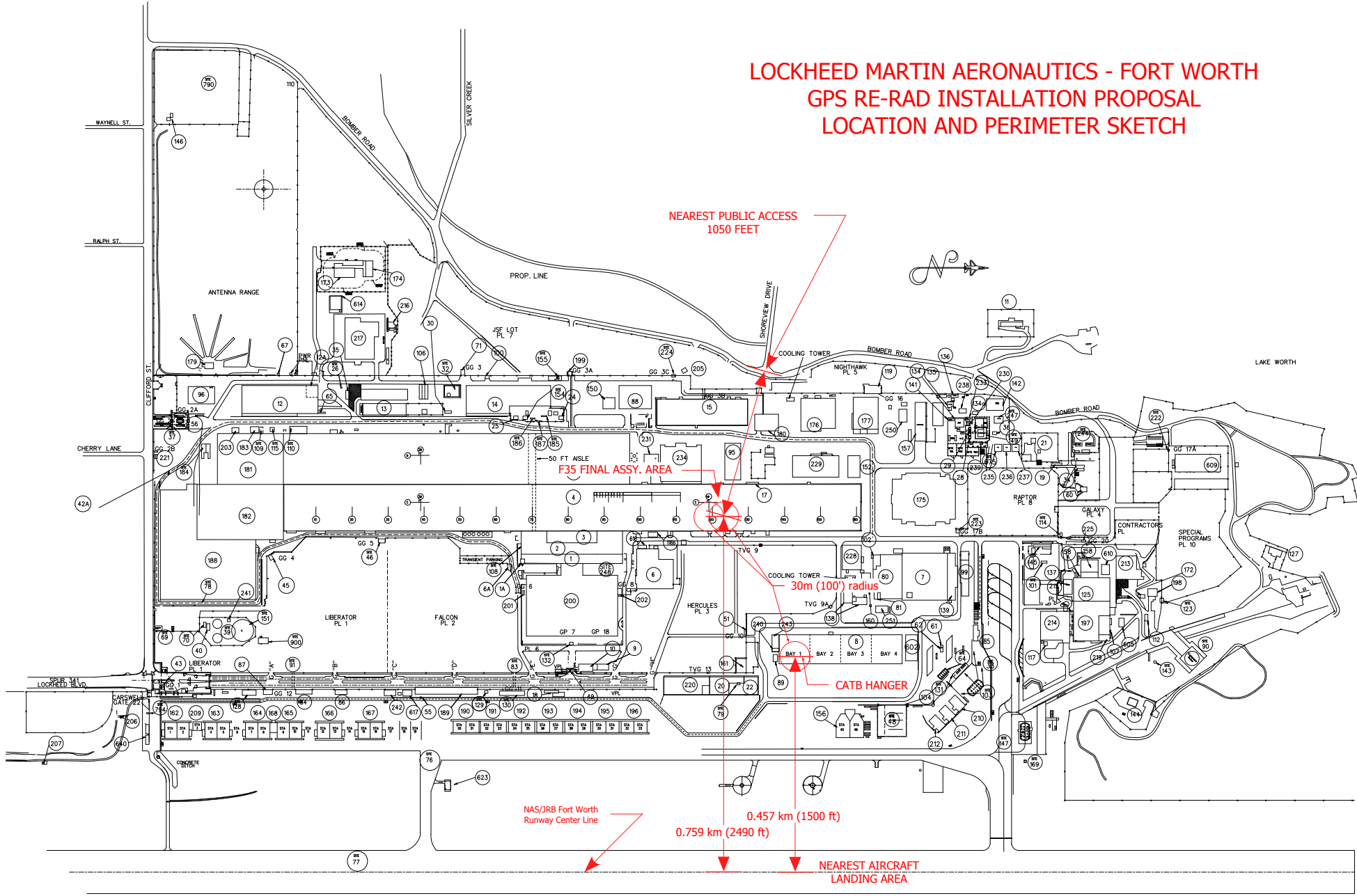
AFP#4 Master Plot Plan by Building Numbers
