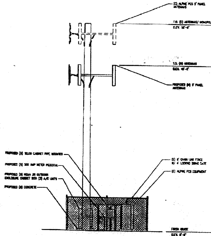
WEST ELEVATION SCALE 1/4"=1'-0"
