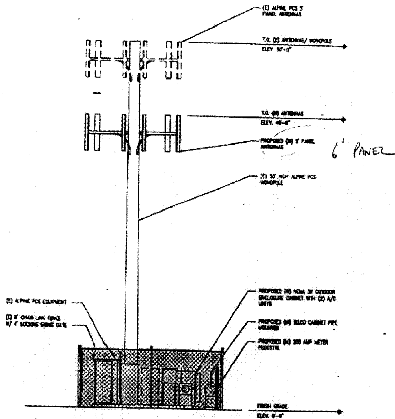
SOUTH ELEVATION SCALE 1/4"=1'-0"
