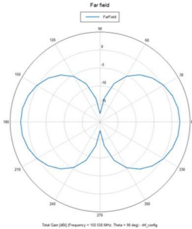
Figure 4-9 - Far field gain (180° is directly above the ADM)
