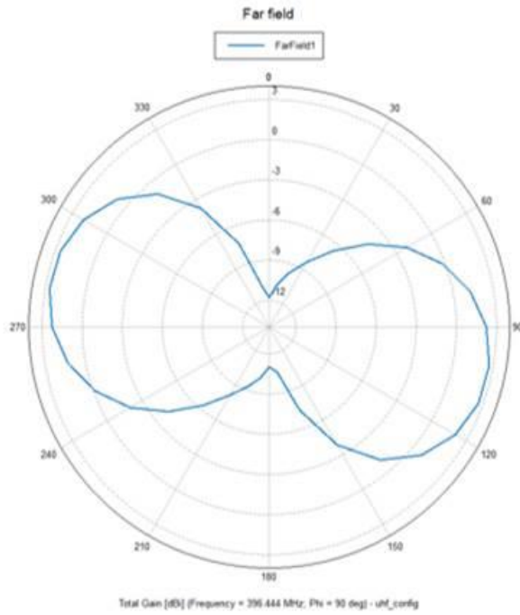
Figure 4-15 - Far field gain (180° is directly above the ADM)
