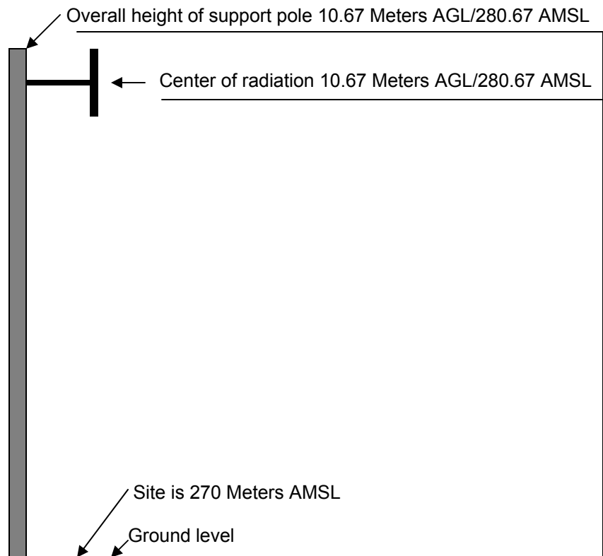
Vertical sketch of antenna and support pole. Not to scale. Channel 201-300 Exhibit # 1
