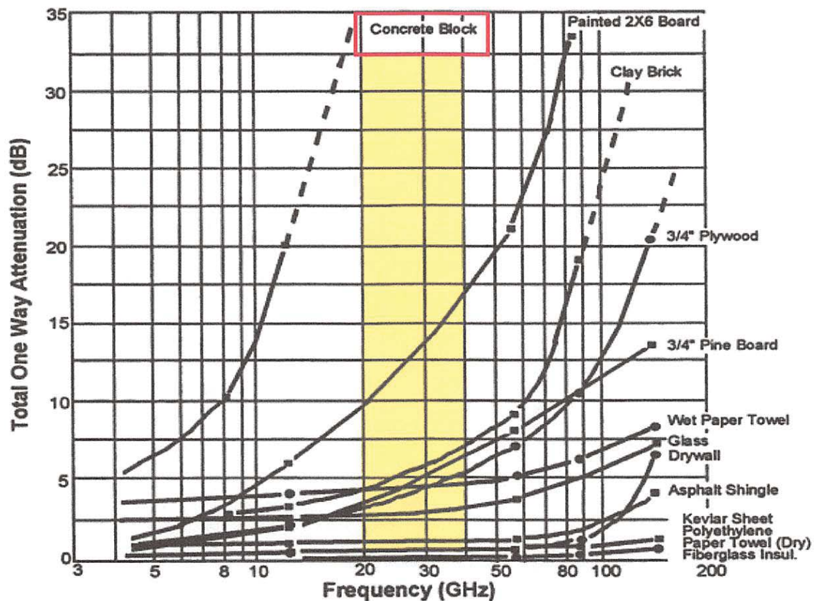
Figure 6: One Way Path Loss of Building Materials versus Frequency 6
