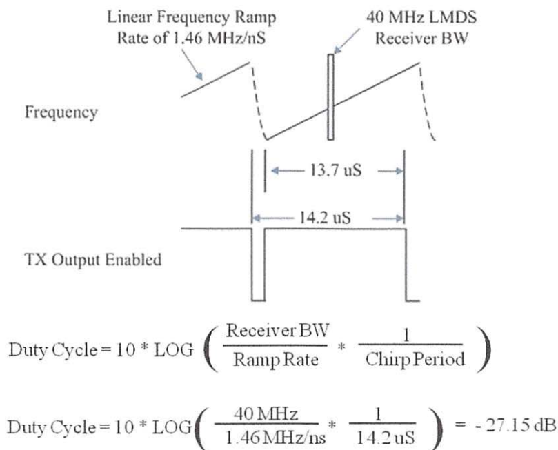
Figure 3: Duty Cycle Calculation for Example 40 MHz Bandwidth Receiver
