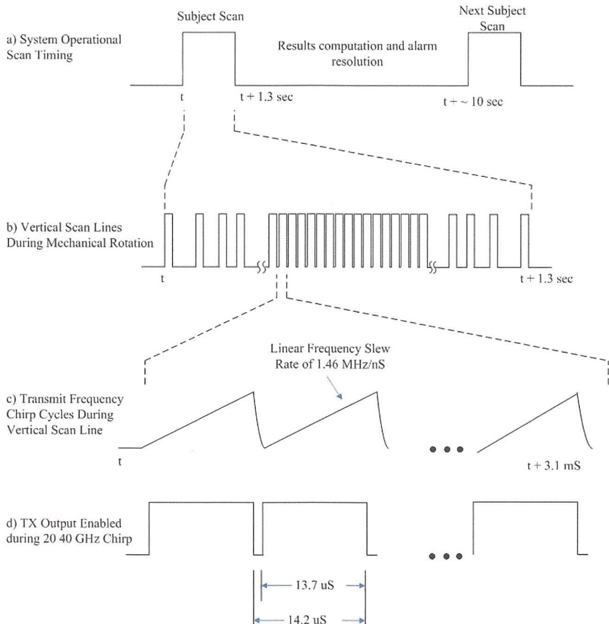
Figure 2: L-3 Next Gen ProVision® System Timing
