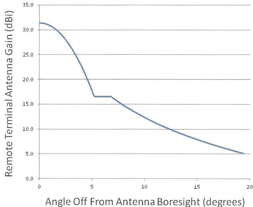
Figure 4: Antenna Gain Calculated for Example Receiver
