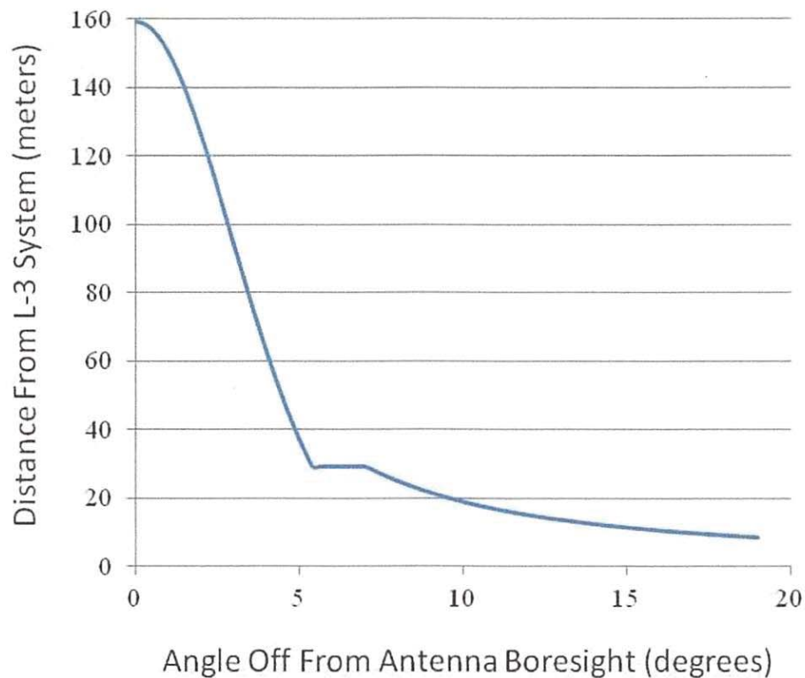
Figure 5: Interfering Distance from LMDS Receiver to L-3 System vs. Angle off LMDS System Boresight
