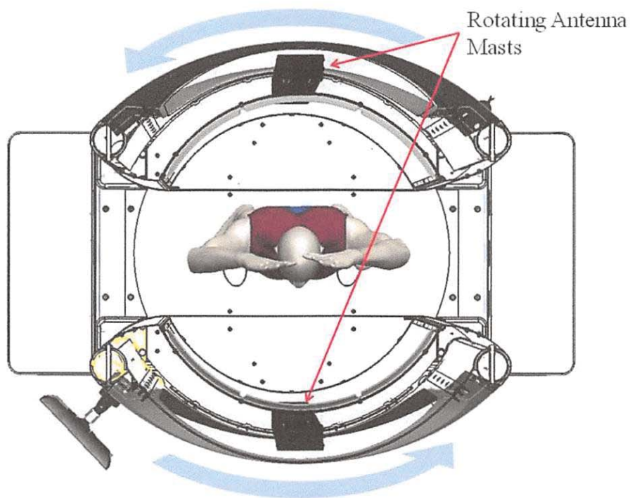
Figure 1: Top View of L-3 System Showing Moving Antenna Masts
