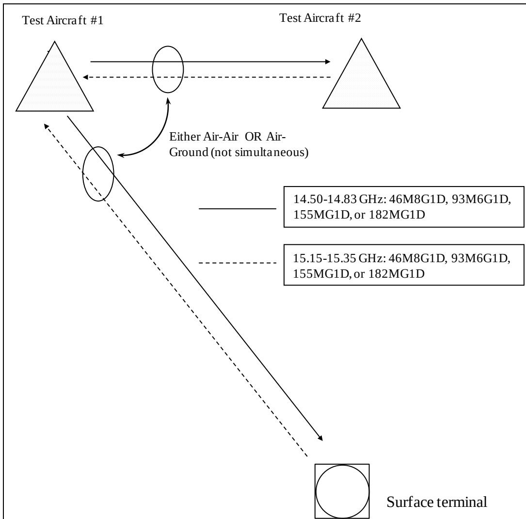
Figure 1. Phase 1 Test Line Diagram, Typical Frequency Plan.
