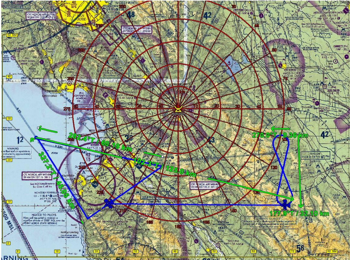
Figure 3. Location of over-land air-to-air testing (scenario 1), south of Hollister, California.
