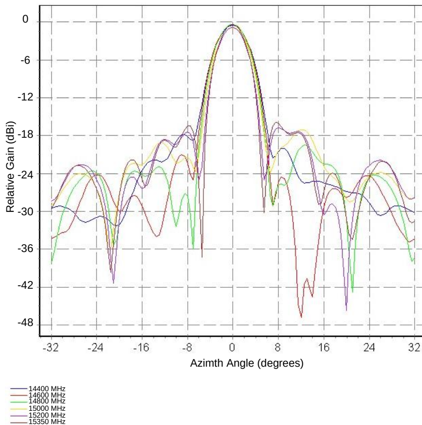
Figure 5. Antenna Pattern
