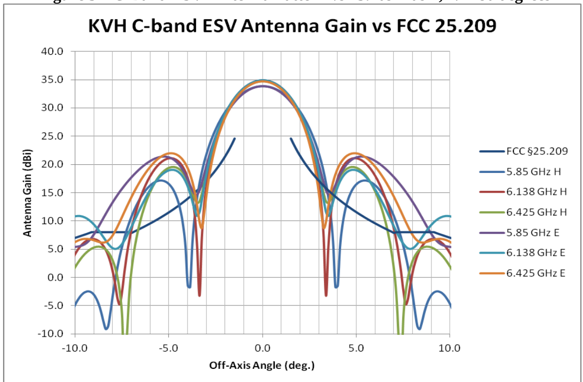
Figure 4– C-band ESV Antenna Pattern vs 25.209 mask , +/- 10 degrees
