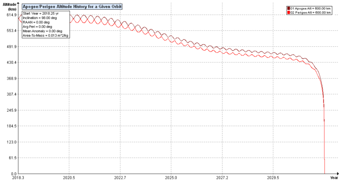
Figure 4. Hamilton-1 orbit history orbit insertion at T=2018.25 , assuming successful antenna deployment.
