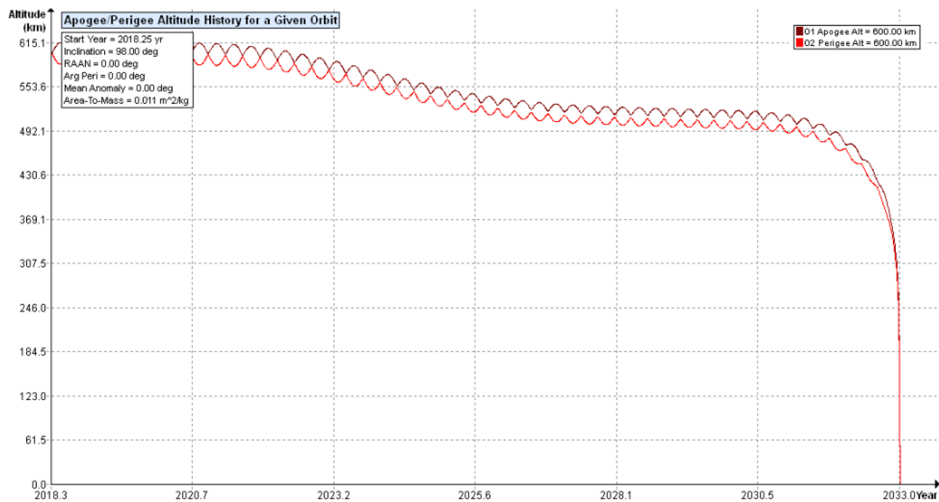
Figure 5. Hamilton-1 orbit history orbit insertion at T=2018.25 , with antenna remaining stowed.
