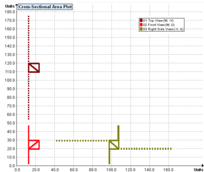
Figure 3. Cross-sectional area plot of Hamilton-1 from DAS with antenna in deployed configuration.
