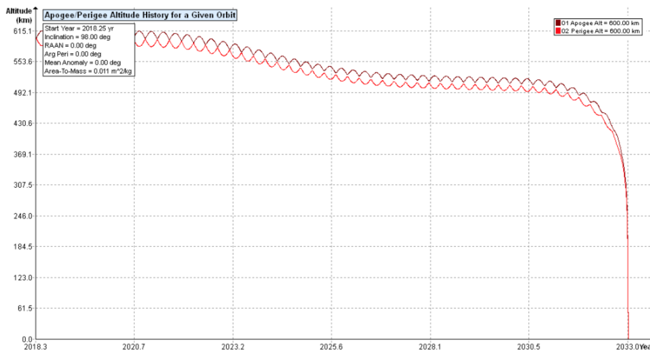
Figure 5. Hamilton-1 orbit history orbit insertion at T=2018.25 , with antenna remaining stowed.
