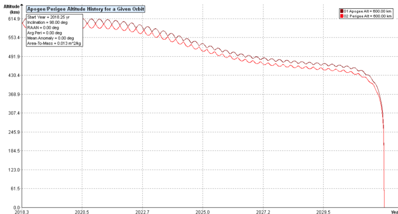
Figure 4. Hamilton-1 orbit history orbit insertion at T=2018.25 , assuming successful antenna deployment.
